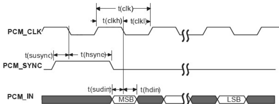
Figure 236: EXT codec to MODULE timing
