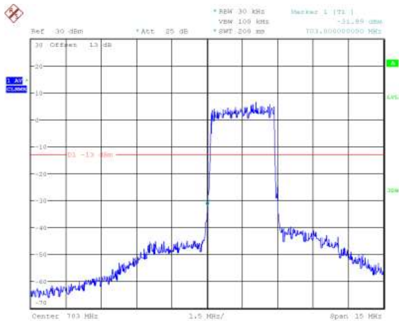
LTE Band28, 3MHz bandwidth, QPSK,(1,0) Mode , Below 703MHz
