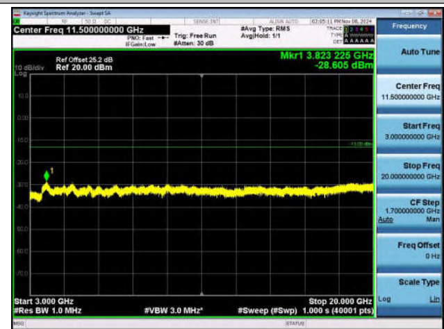
Band25_20MHz_QPSK_26590_1RB#0_3000~20000_3000~20000
