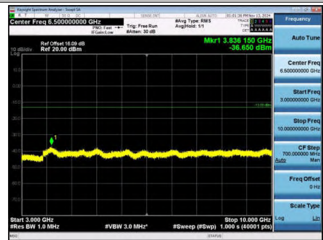
Band26_15MHz_QPSK_26915_1RB#0_3000~10000_3000~10000
