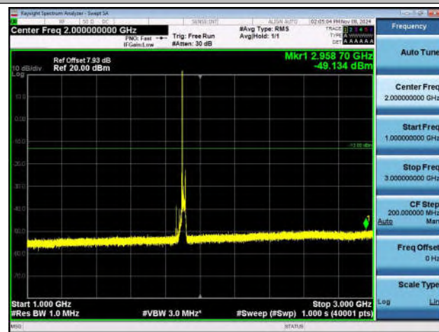
Band25_20MHz_QPSK_26590_1RB#0_1000~3000_1000~3000
