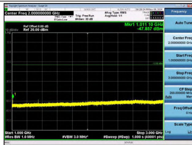
Band71_20MHz_QPSK_133322_1RB#0_1000~3000_1000
