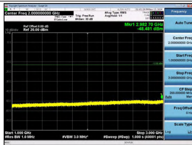
Band26_15MHz_QPSK_26915_1RB#0_1000~3000_1000~3000
