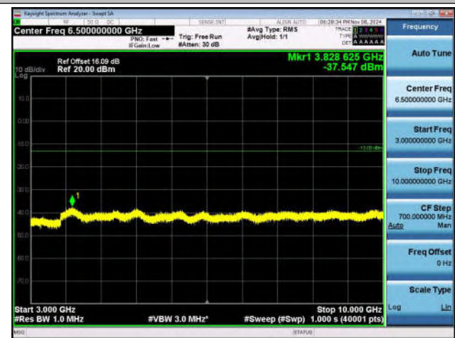
Band71_20MHz_QPSK_133322_1RB#0_3000~10000_300
