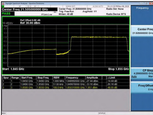
Band25_10MHz_QPSK_26090_50RB#0
