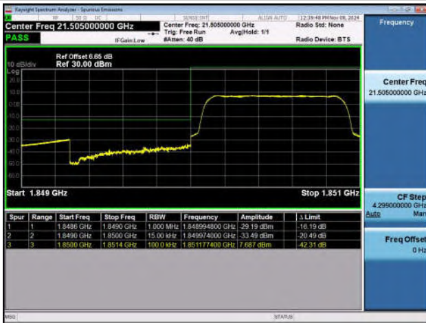
Band25_3MHz_QPSK_26055_1RB#14
