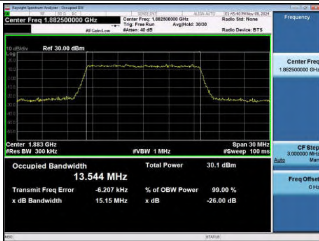
Band25-15MHz-QPSK-26365-75RB#0-PASS
