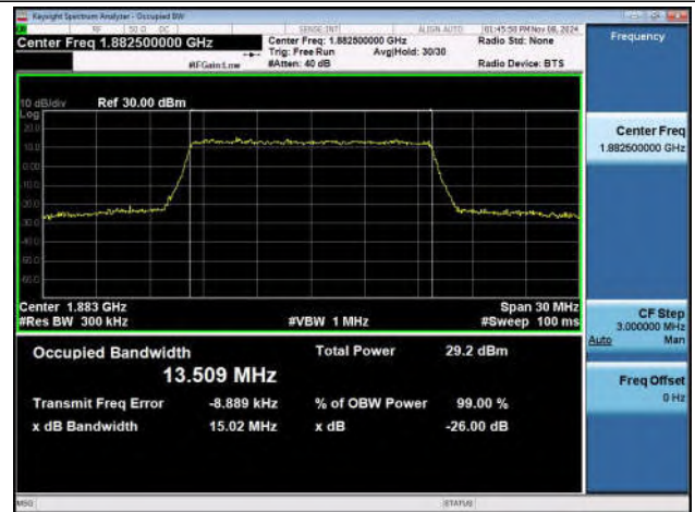
Band25-15MHz-16QAM-26365-75RB#0-PASS
