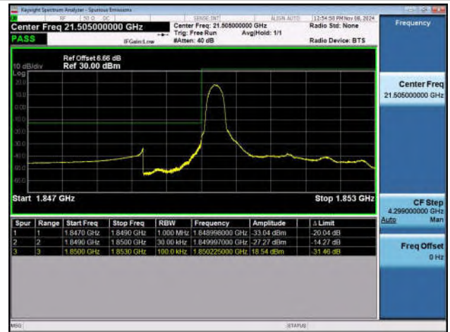
Band25_3MHz_QPSK_26055_15RB#0
