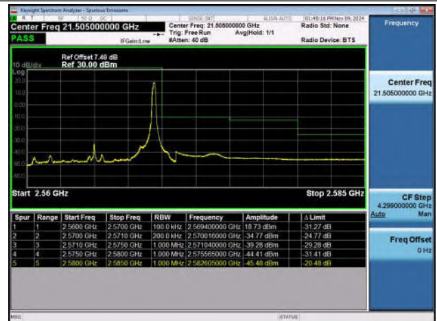
Band7_10MHz_QPSK_21400_1RB#49
