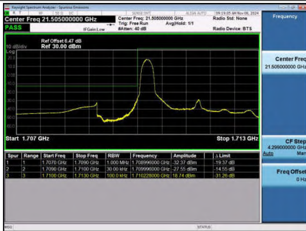
Band4_3MHz_QPSK_19965_1RB#0
