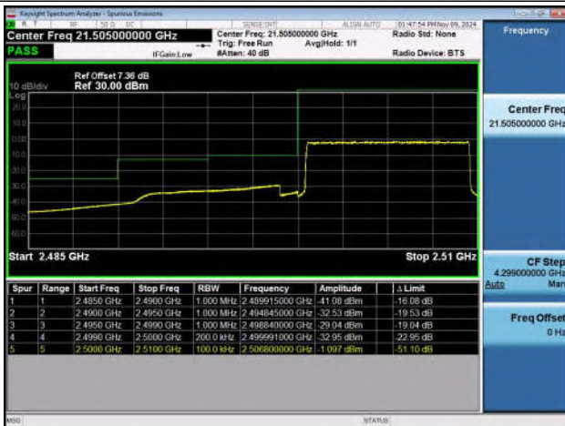
Band7_10MHz_QPSK_20800_50RB#0
