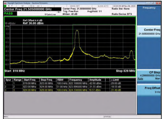
Band5_5MHz_QPSK_20625_1RB#24
