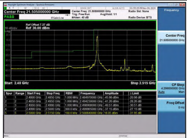
Band7_15MHz_QPSK_21375_1RB#74
