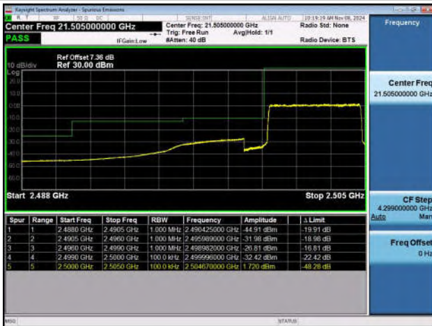
Band7_5MHz_QPSK_21425_25RB#0
