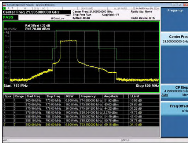
Band13_5MHz_QPSK_23255_25RB#0
