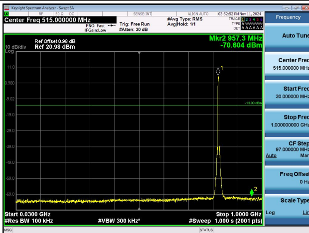
Band5-4183-30~1000MHz-PASS
