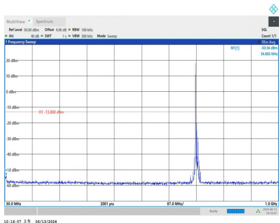
Band17_10MHz_QPSK_23790_1RB#0_30~1000_30~1000
