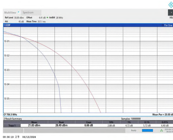
Band17-5MHz-16QAM-23755-25RB#0-PASS
