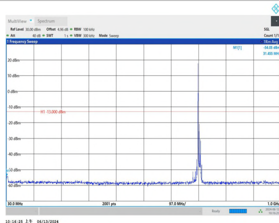
Band17_10MHz_QPSK_23800_1RB#0_30~1000_30~1000
