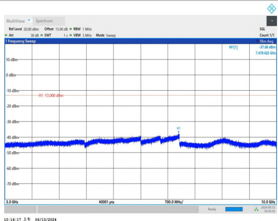
Band17_10MHz_QPSK_23790_1RB#0_3000~10000_3000~10000
