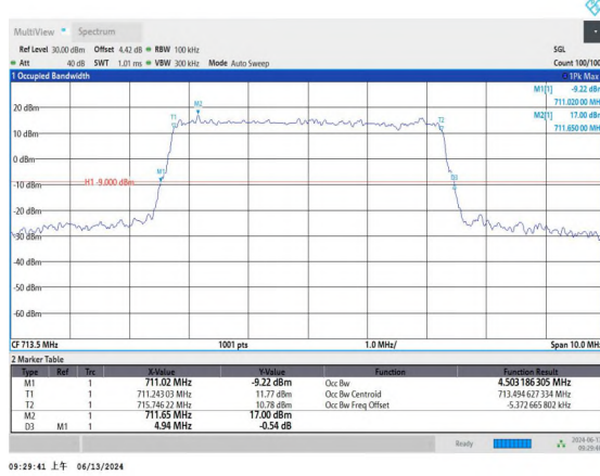
Band17-5MHz-QPSK-23825-25RB#0-PASS
