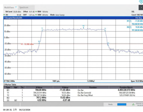
Band17-5MHz-16QAM-23755-25RB#0-PASS
