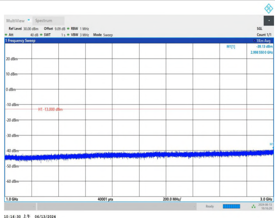
Band17_10MHz_QPSK_23800_1RB#0_1000~3000_1000~3000
