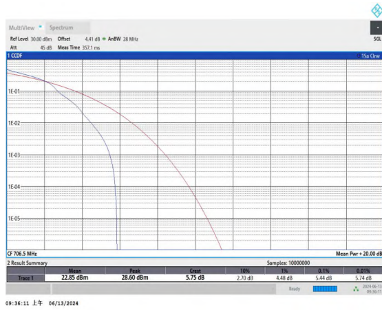
Band17-5MHz-16QAM-23755-1RB#0-PASS
