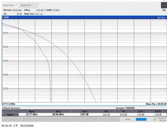
Band17-10MHz-16QAM-23800-1RB#0-PASS
