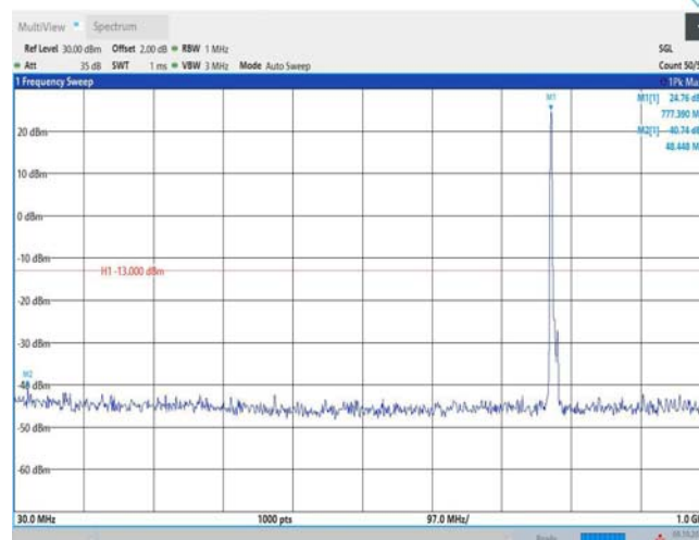
Band13-5MHz-QPSK-23205-1RB#0-Range1:30~1000MHz
