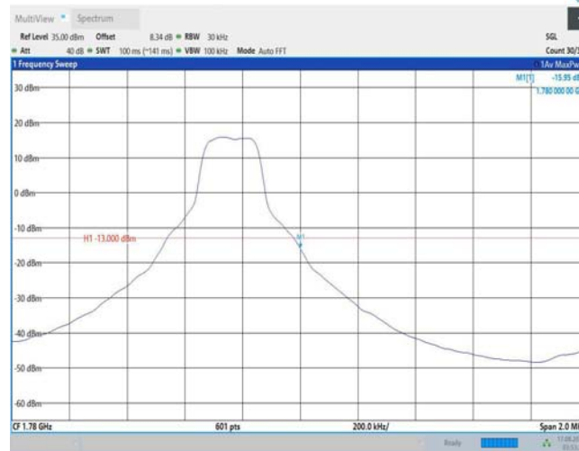
Band66-3MHz-16QAM-132657-15RB#0
