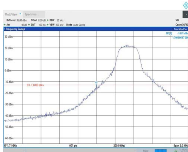
Band66-5MHz-16QAM-131997-1RB#24
