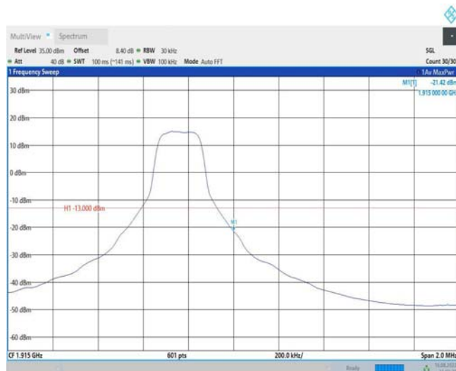
Band25-3MHz-QPSK-26675-15RB#0
