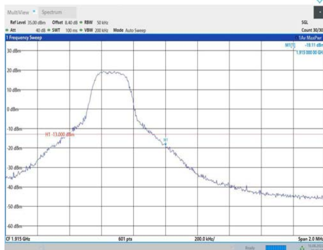
Band25-5MHz-QPSK-26665-25RB#0
