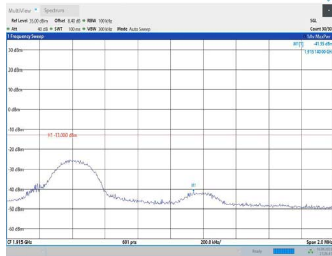
Band25-10MHz-16QAM-26640-1RB#49
