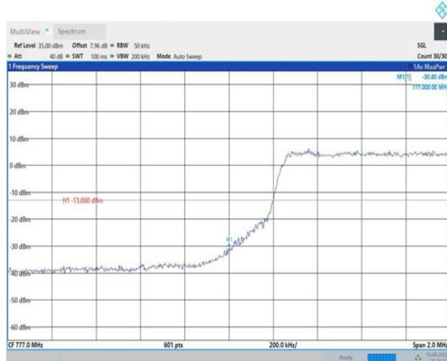
Band13-5MHz-16QAM-23255-1RB#0
