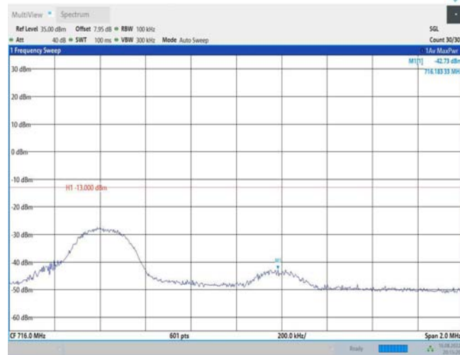
Band12-10MHz-16QAM-23130-1RB#49
