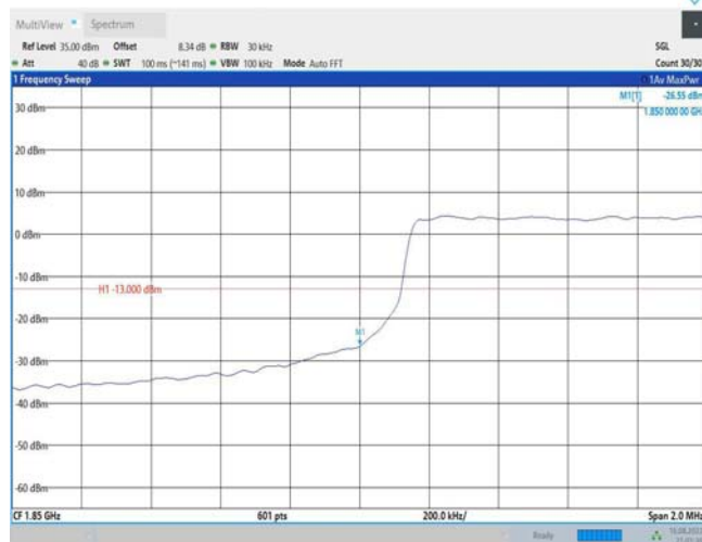
Band25-3MHz-QPSK-26675-1RB#0
