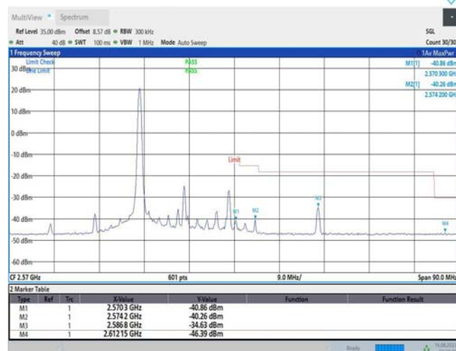
Band7-20MHz-16QAM-21350-1RB#99
