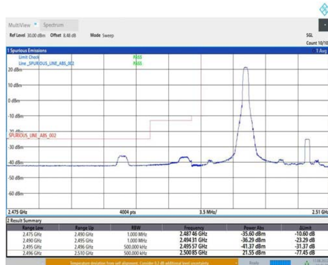
Band7-15MHz-16QAM-20825-1RB#74
