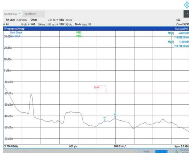
Band12-1.4MHz-QPSK-23173-1RB#5
