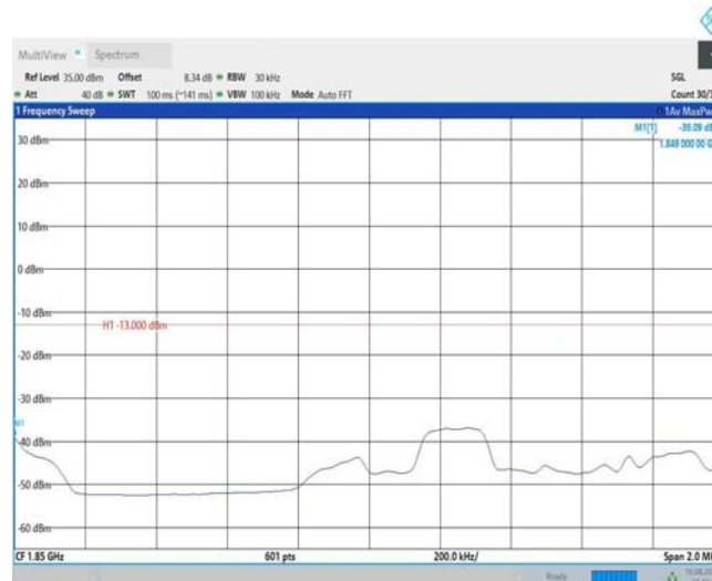
Band25-3MHz-16QAM-26055-15RB#0
