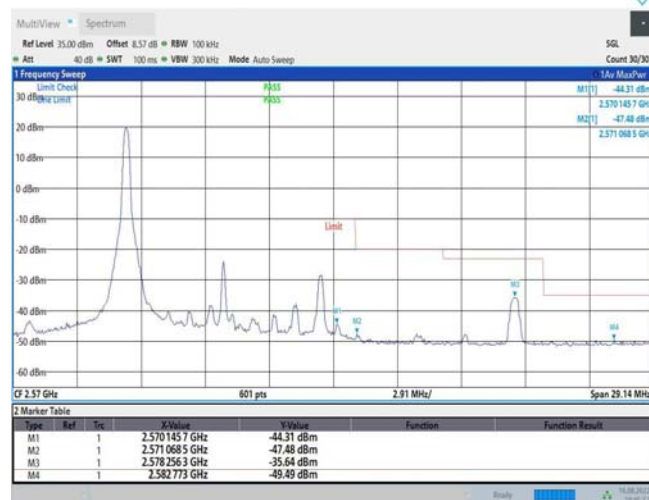
Band7-10MHz-QPSK-21400-1RB#49
