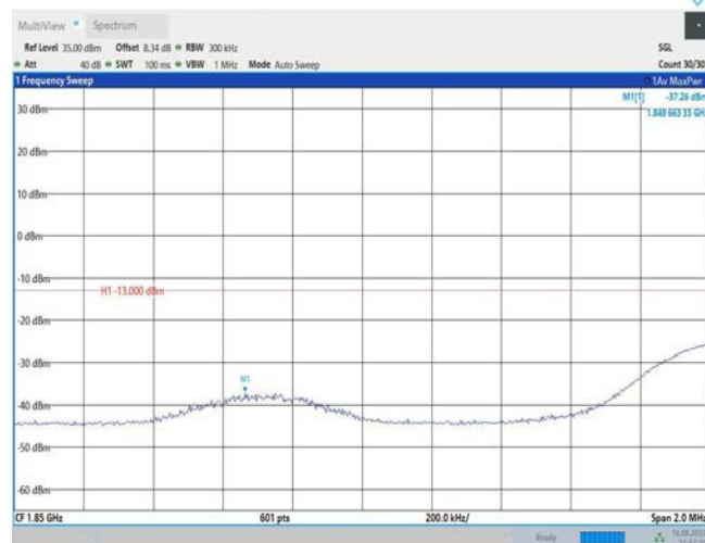
Band25-20MHz-QPSK-26140-100RB#0
