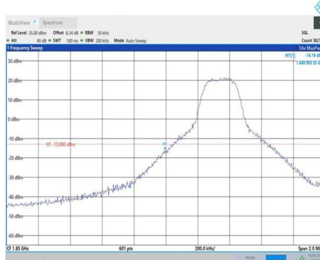
Band25-5MHz-16QAM-26065-1RB#24
