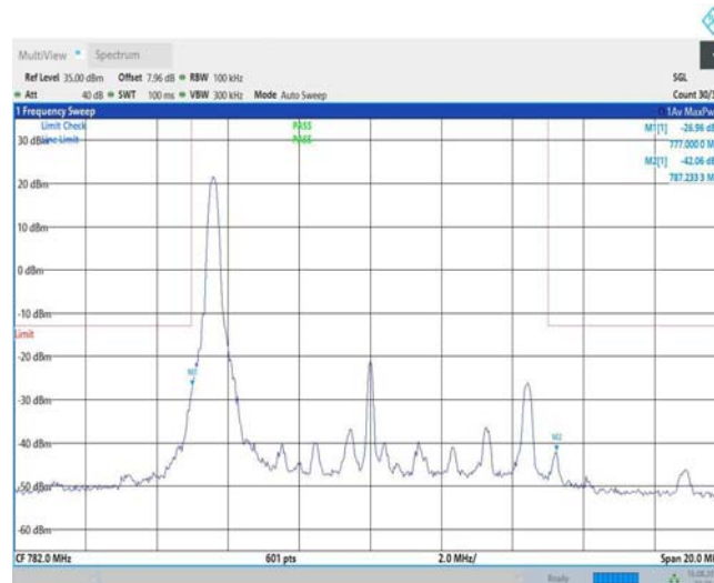
Band13-10MHz-16QAM-23230-1RB#49
