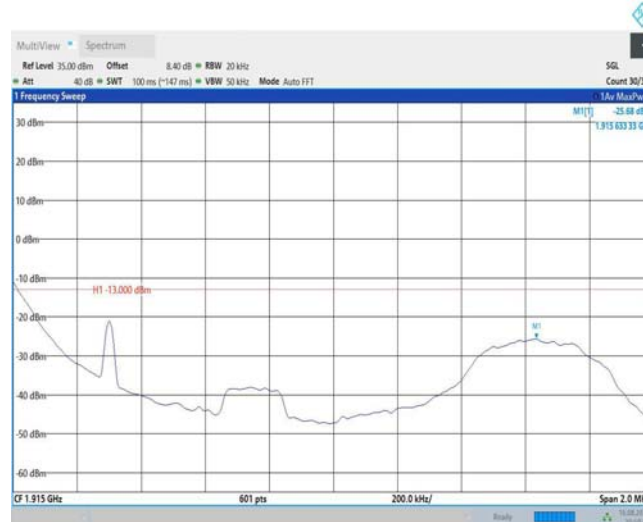
Band25-1.4MHz-16QAM-26683-1RB#5
