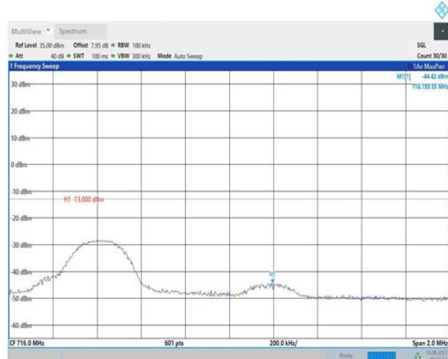
Band12-10MHz-QPSK-23130-1RB#49
