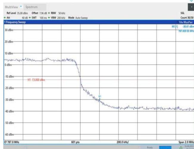
Band13-10MHz-QPSK-23230-1RB#0
