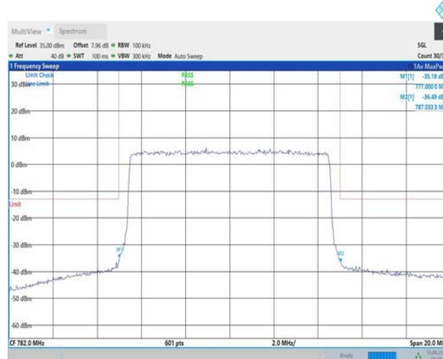
Band13-10MHz-16QAM-23230-1RB#0
