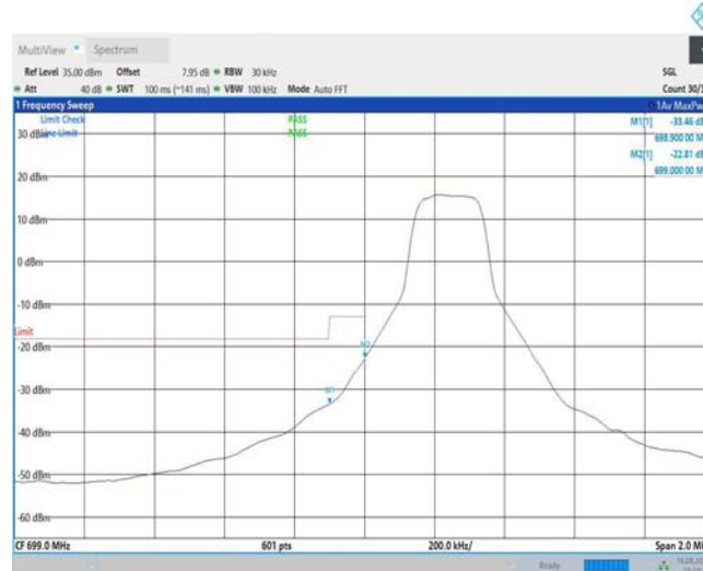
Band12-3MHz-QPSK-23025-1RB#14
