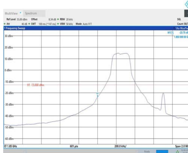
Band25-1.4MHz-QPSK-26047-1RB#5
