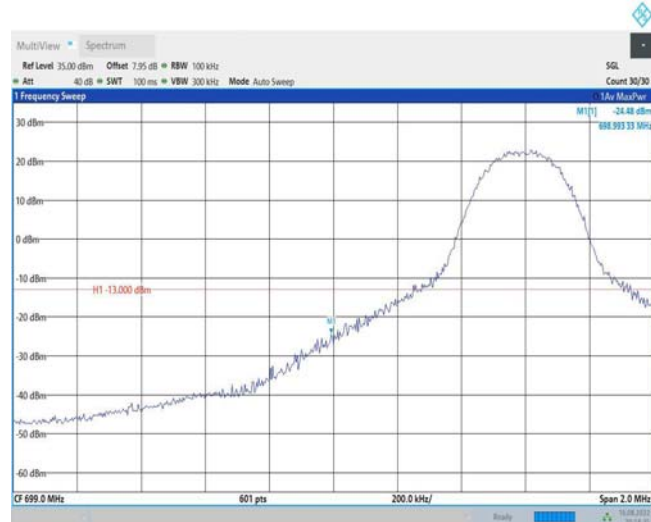
Band12-10MHz-16QAM-23060-1RB#49
