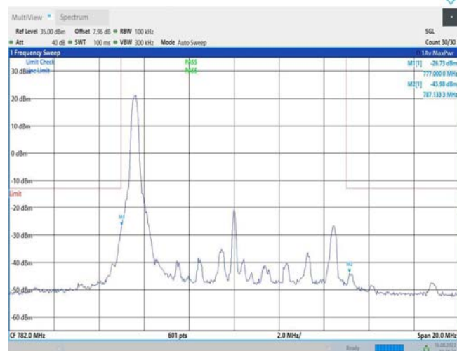
Band13-10MHz-QPSK-23230-1RB#49
