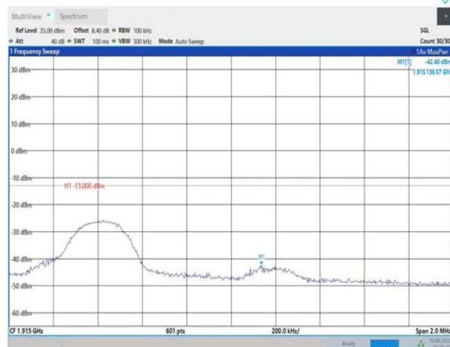
Band25-10MHz-QPSK-26640-1RB#49
