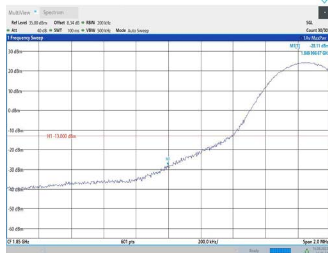
Band25-15MHz-16QAM-26115-1RB#74
