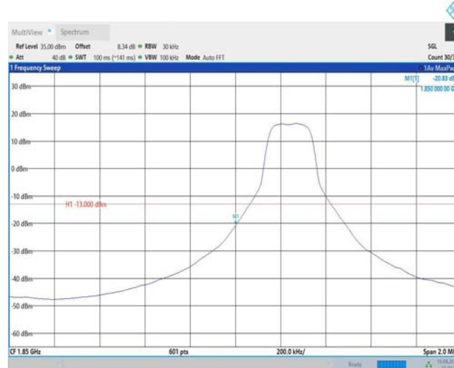
Band25-3MHz-16QAM-26055-1RB#14
