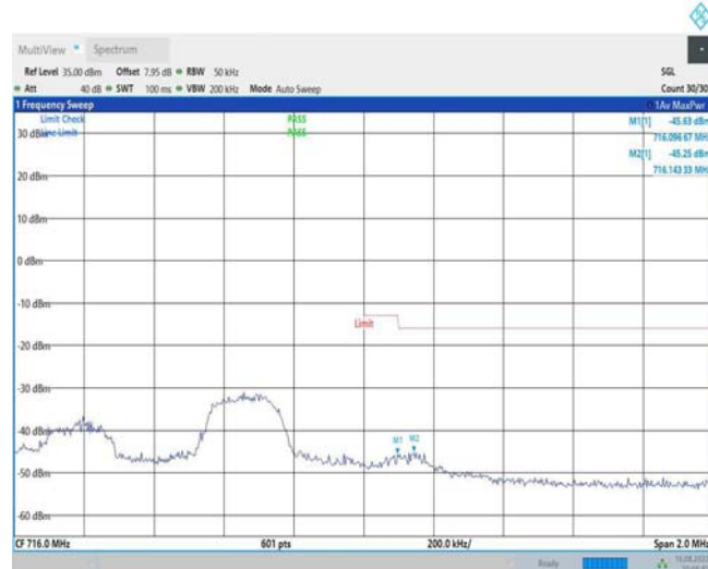
Band12-5MHz-QPSK-23155-1RB#24
