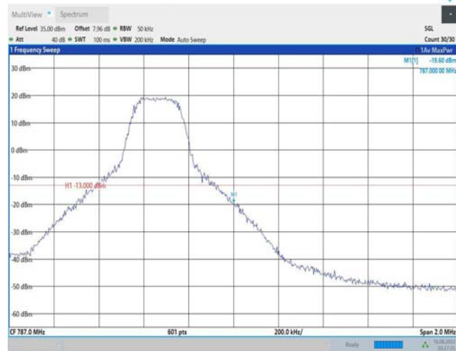
Band13-5MHz-16QAM-23255-25RB#0
