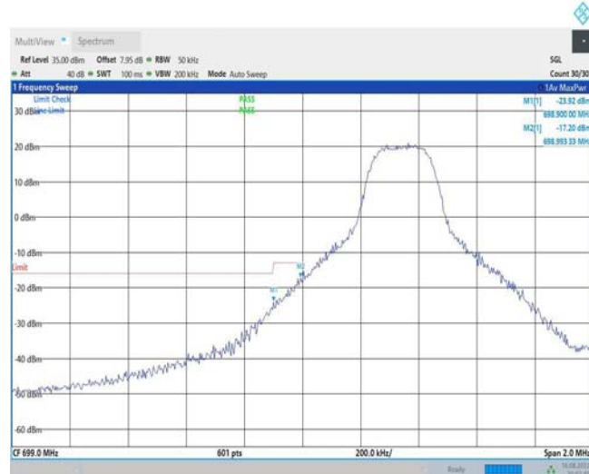
Band12-5MHz-16QAM-23035-1RB#24
