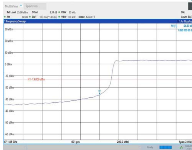
Band25-3MHz-16QAM-26675-1RB#0
