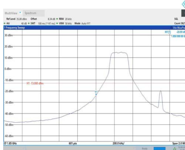
Band25-1.4MHz-16QAM-26047-1RB#5
