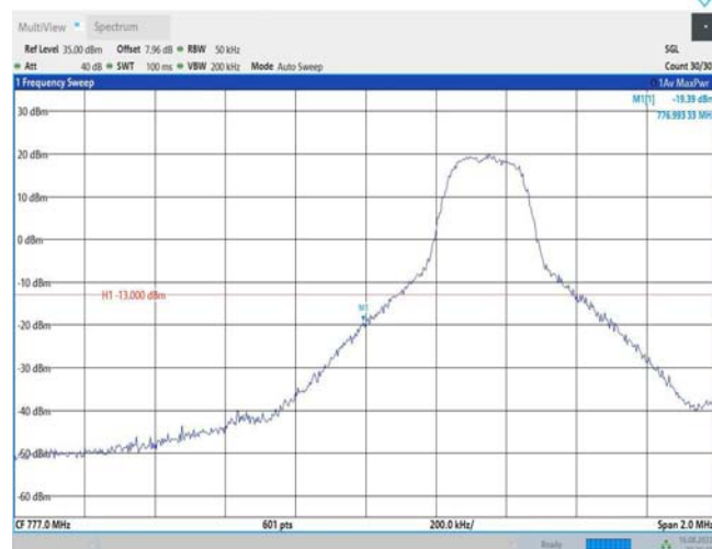
Band13-5MHz-QPSK-23205-1RB#24
