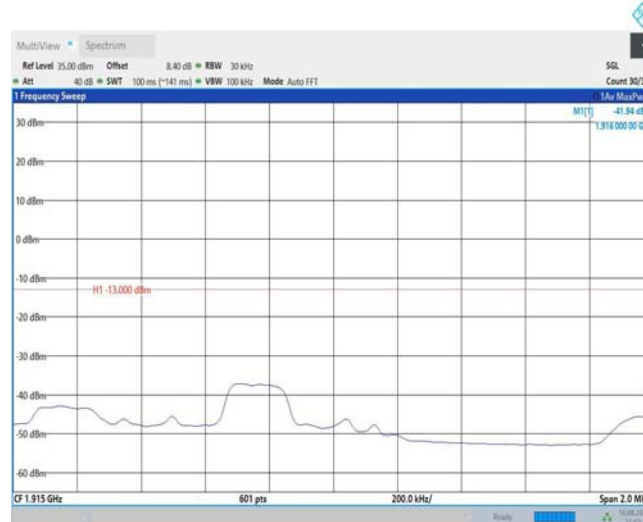
Band25-3MHz-16QAM-26675-1RB#14
