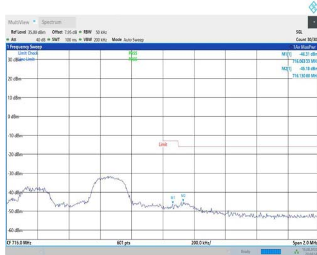
Band12-5MHz-16QAM-23155-1RB#24
