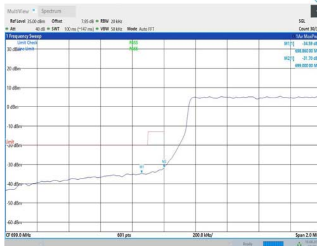
Band12-1.4MHz-16QAM-23173-1RB#0
