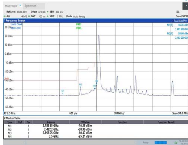
Band7-20MHz-16QAM-20850-1RB#99
