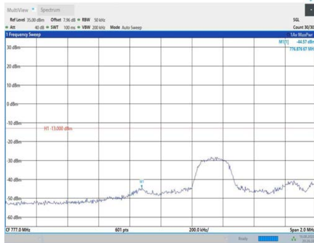
Band13-5MHz-16QAM-23205-25RB#0
