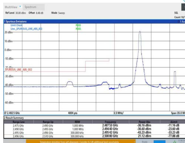
Band7-15MHz-QPSK-20825-1RB#74
