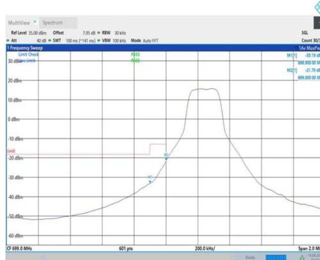
Band12-3MHz-16QAM-23025-1RB#14
