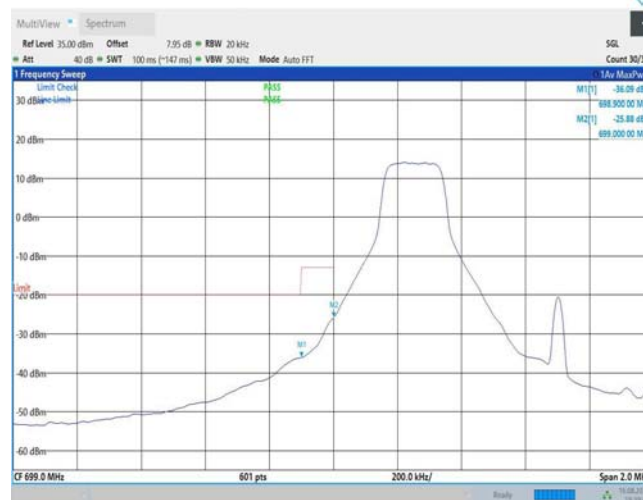
Band12-1.4MHz-QPSK-23017-1RB#5
