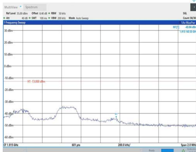
Band25-5MHz-QPSK-26665-1RB#24
