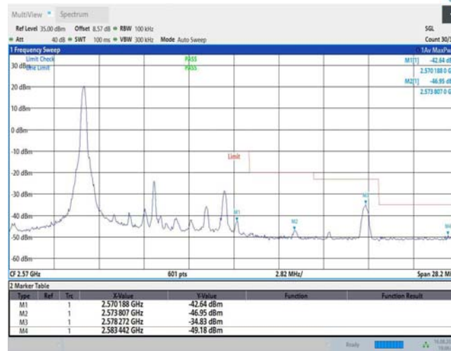
Band7-10MHz-16QAM-21400-1RB#49
