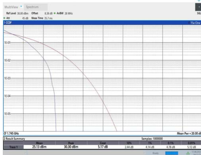
Band66-5MHz-QPSK-132322-25RB#0
