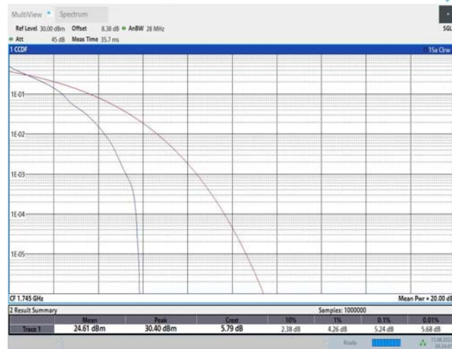
Band66-15MHz-QPSK-132322-75RB#0
