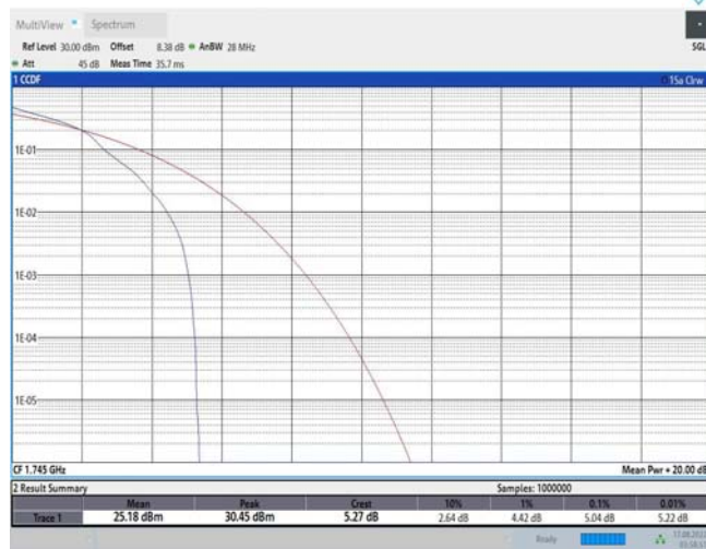
Band66-3MHz-16QAM-132322-15RB#0
