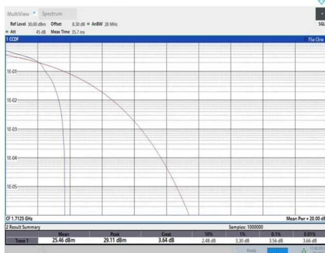
Band66-5MHz-16QAM-131997-25RB#0
