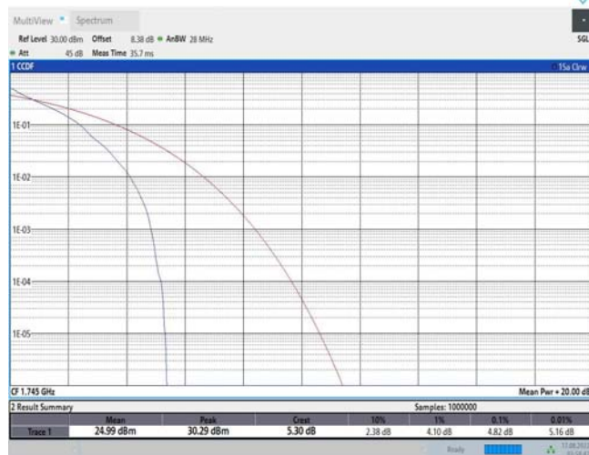
Band66-3MHz-QPSK-132322-15RB#0
