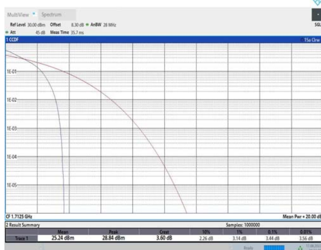
Band66-5MHz-QPSK-132322-1RB#0
