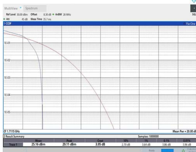
Band66-3MHz-16QAM-131987-15RB#0
