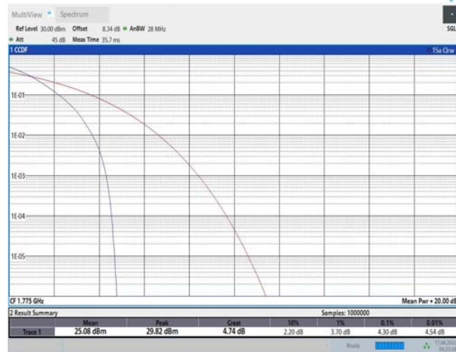
Band66-10MHz-16QAM-132022-1RB#0
