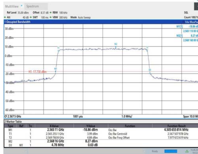
Band7-5MHz-16QAM-20775-25RB#0
