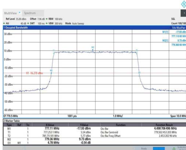
Band13-5MHz-QPSK-23230-25RB#0
