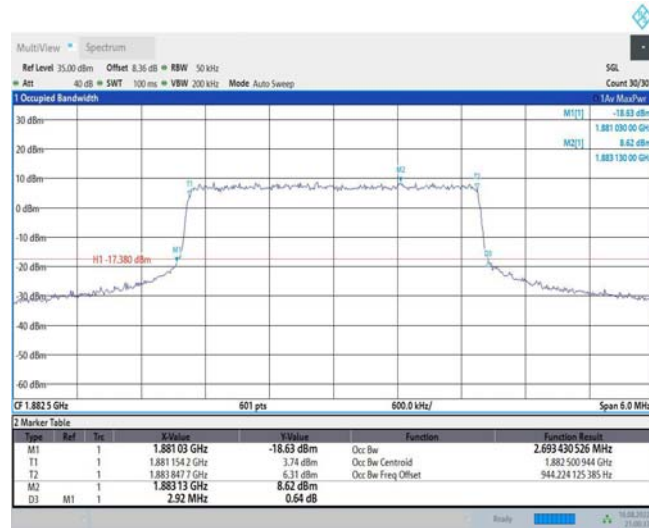
Band25-3MHz-16QAM-26675-15RB#0
