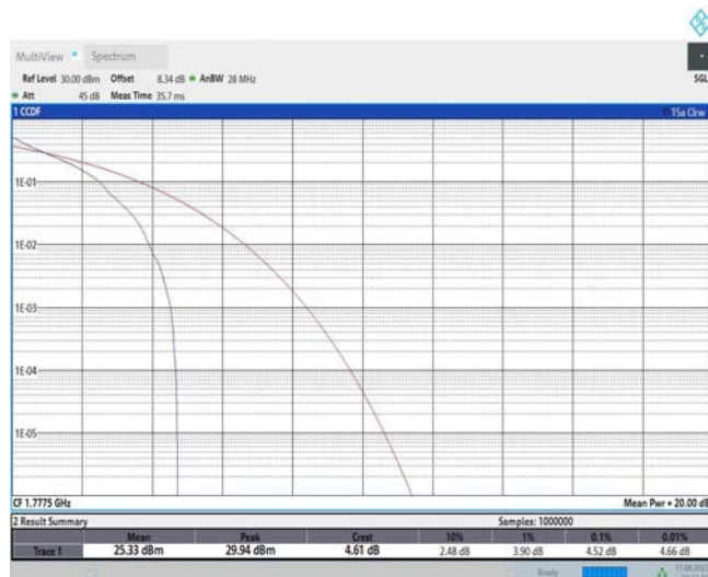
Band66-5MHz-QPSK-132647-25RB#0
