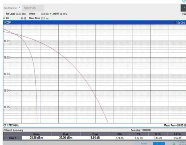
Band66-15MHz-QPSK-132047-75RB#0
