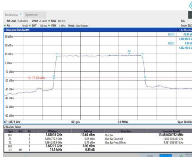
Band25-15MHz-QPSK-26365-75RB#0
