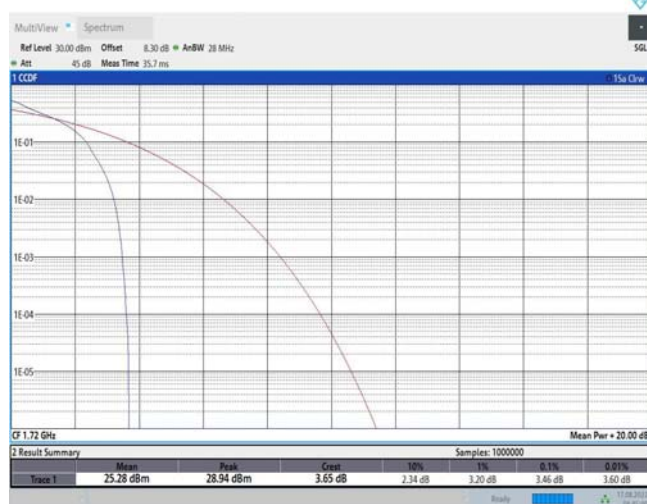
Band66-20MHz-QPSK-132072-100RB#0
