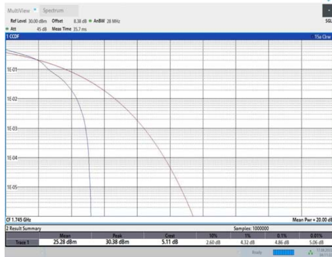
Band66-5MHz-16QAM-132322-25RB#0
