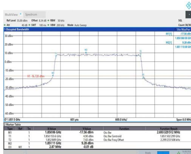
Band25-3MHz-16QAM-26365-15RB#0
