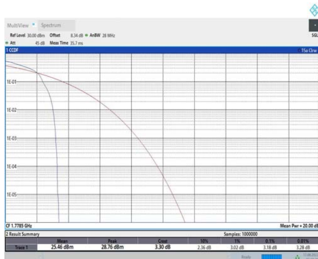
Band66-3MHz-16QAM-132657-15RB#0
