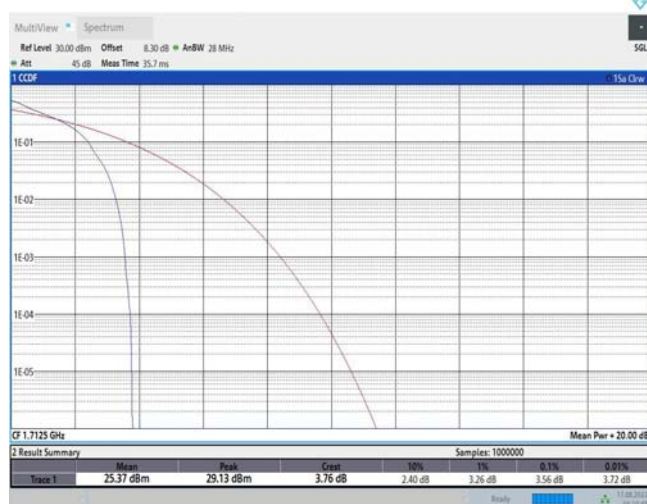
Band66-5MHz-QPSK-131997-25RB#0
