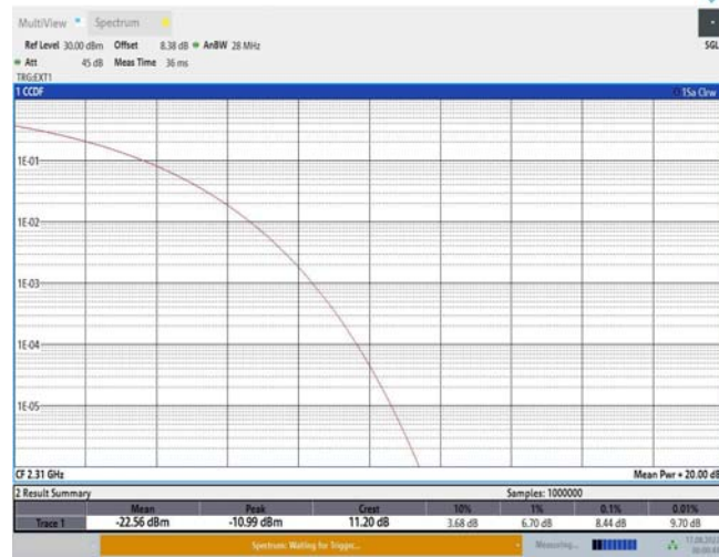
Band40-5MHz-16QAM-38750-25RB#0
