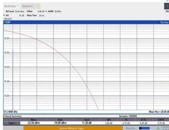
Band41-5MHz-16QAM-39675-25RB#0
