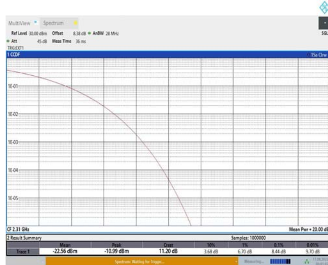
Band40-5MHz-16QAM-38775-1RB#0
