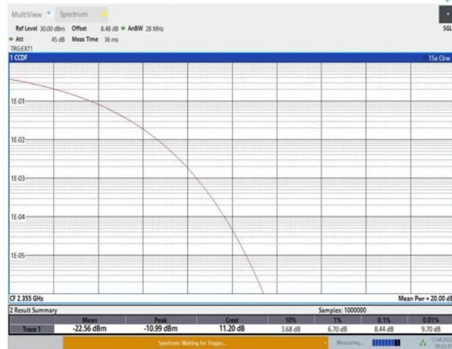
Band40-5MHz-16QAM-39200-25RB#0
