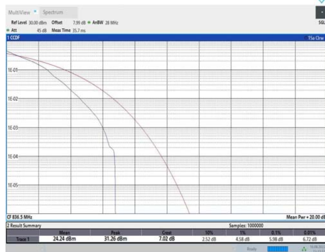
Band26-10MHz-QPSK-26915-50RB#0
