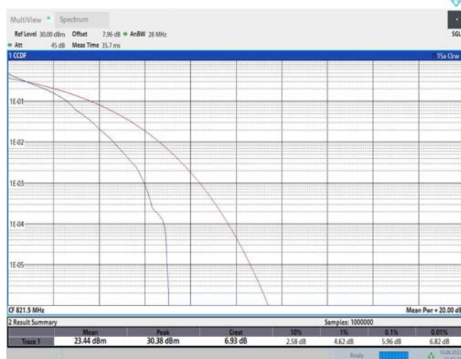
Band26-15MHz-QPSK-26765-75RB#0
