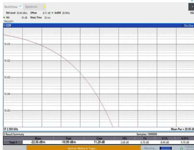
Band41-10MHz-QPSK-40620-50RB#0
