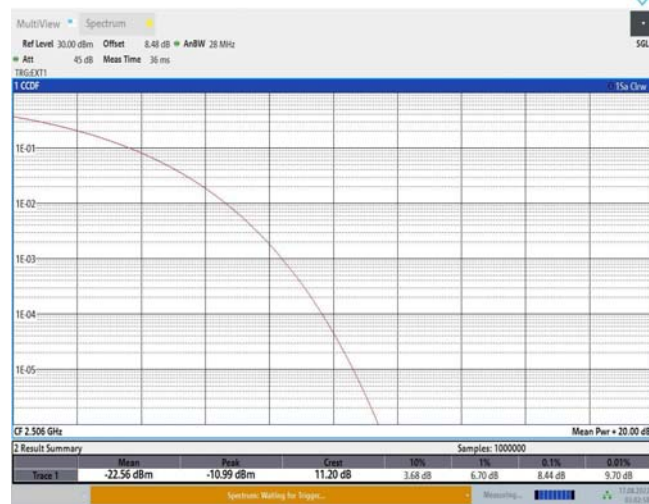
Band41-20MHz-QPSK-39750-100RB#0
