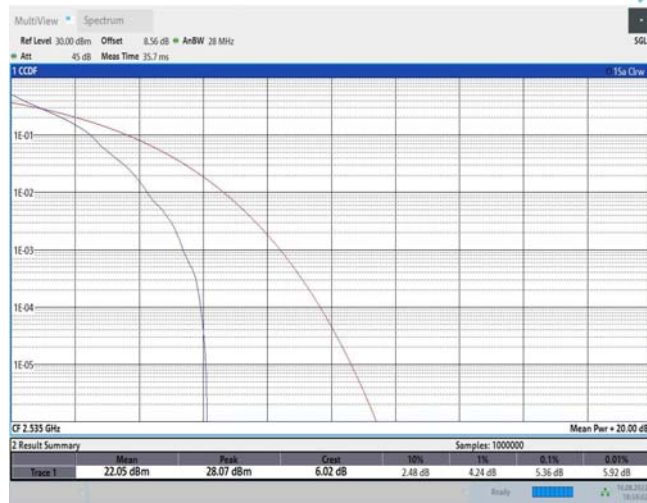
Band7-5MHz-QPSK-21100-25RB#0
