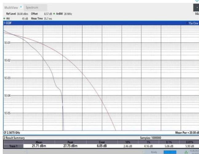
Band7-5MHz-QPSK-21425-25RB#0
