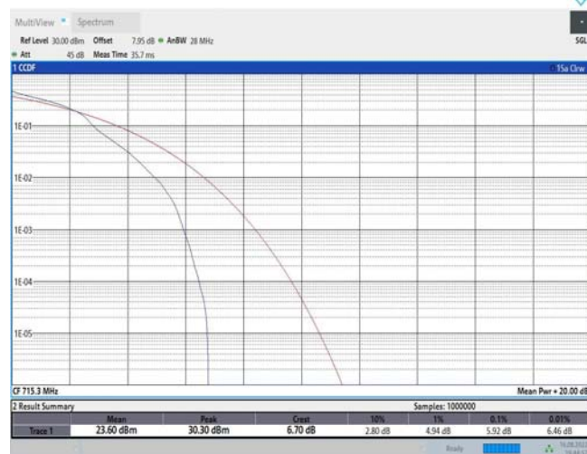
Band12-1.4MHz-16QAM-23173-6RB#0
