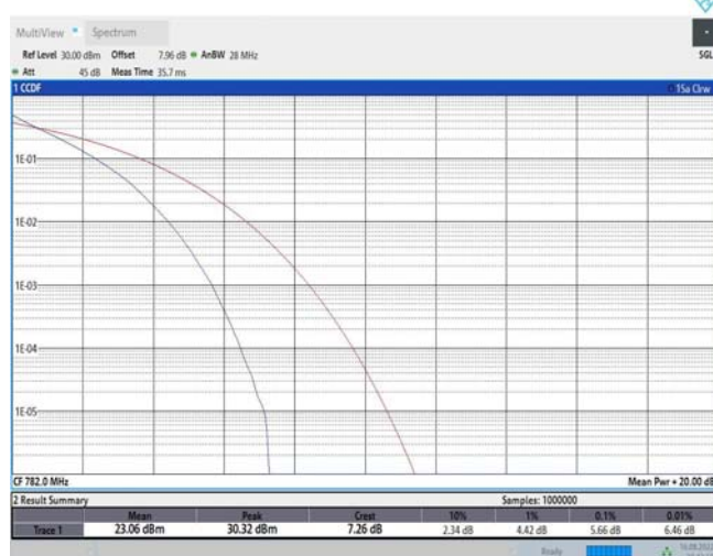
Band13-10MHz-16QAM-23230-1RB#0
