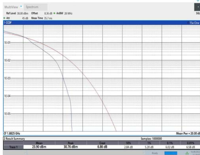
Band25-5MHz-16QAM-26365-25RB#0
