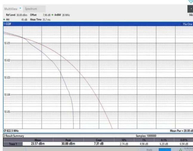
Band26-3MHz-16QAM-26775-15RB#0
