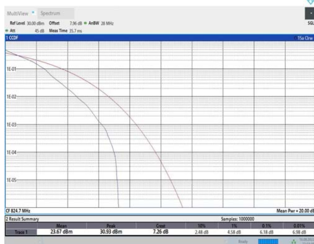
Band26-1.4MHz-QPSK-26797-6RB#0
