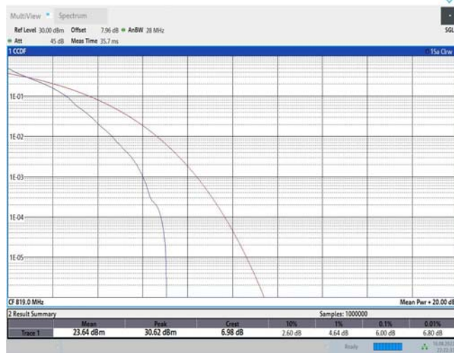
Band26-3MHz-QPSK-26740-15RB#0
