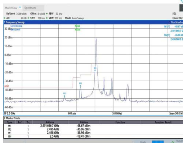
Band7-5MHz-16QAM-20775-1RB#24
