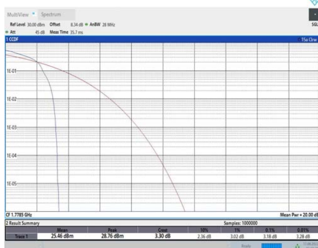
Band66-3MHz-16QAM-132657-15RB#0
