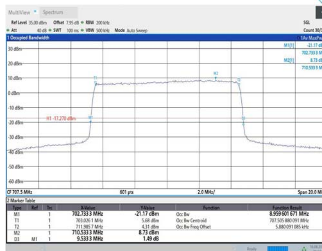
Band12-10MHz-QPSK-23130-50RB#0
