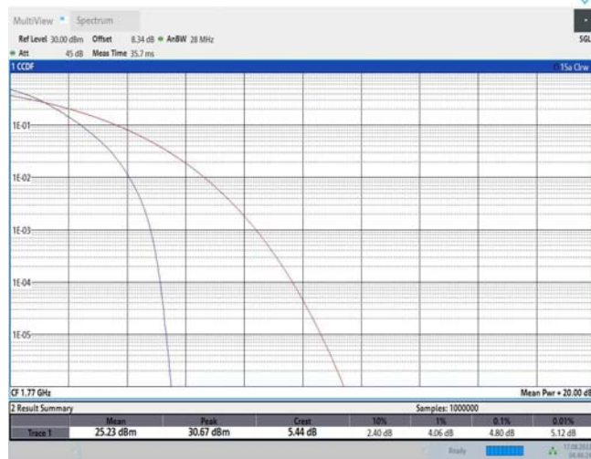
Band66-20MHz-16QAM-132072-1RB#0
