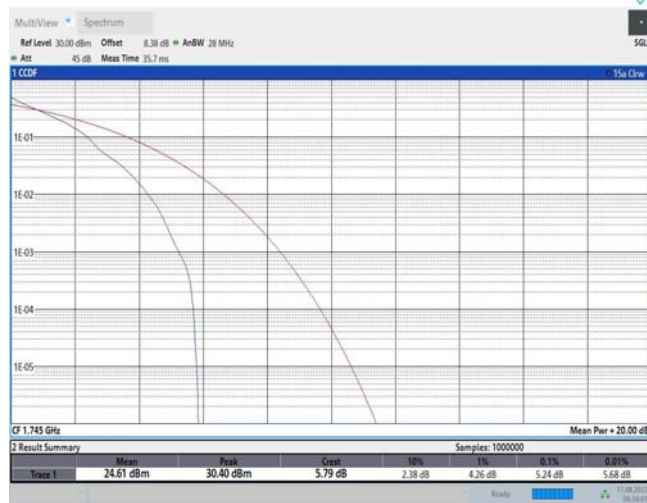
Band66-15MHz-QPSK-132322-75RB#0
