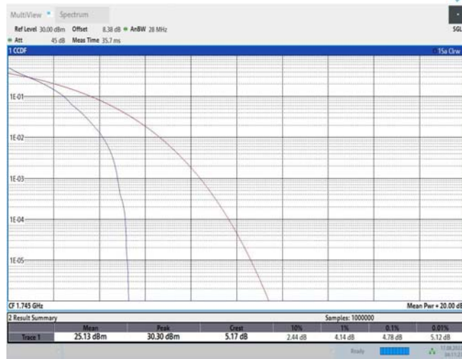
Band66-5MHz-QPSK-132322-25RB#0
