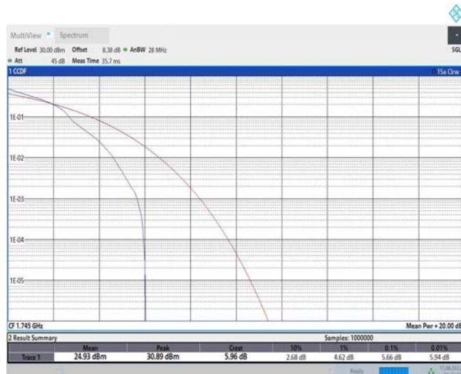
Band66-10MHz-16QAM-132622-1RB#0
