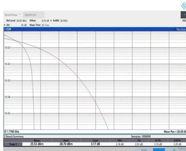
Band66-3MHz-QPSK-132657-15RB#0
