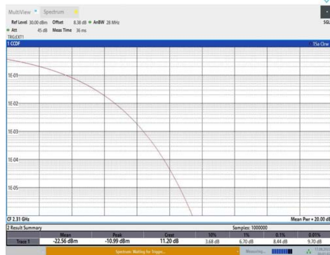
Band40-5MHz-16QAM-38775-1RB#0
