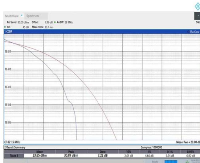
Band26-5MHz-QPSK-26765-25RB#0
