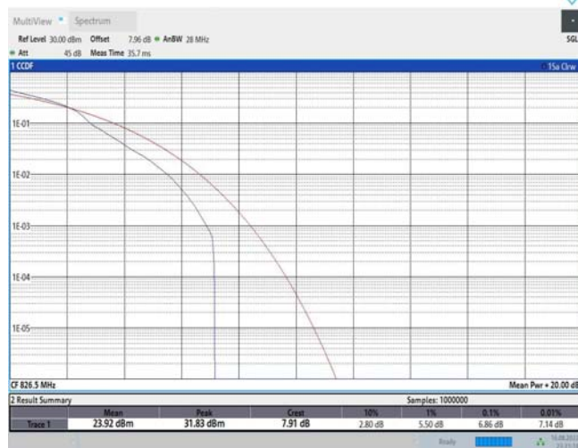
Band26-5MHz-16QAM-26815-25RB#0
