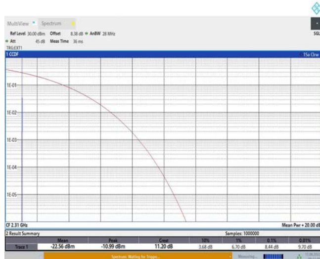
Band40-10MHz-QPSK-38750-50RB#0
