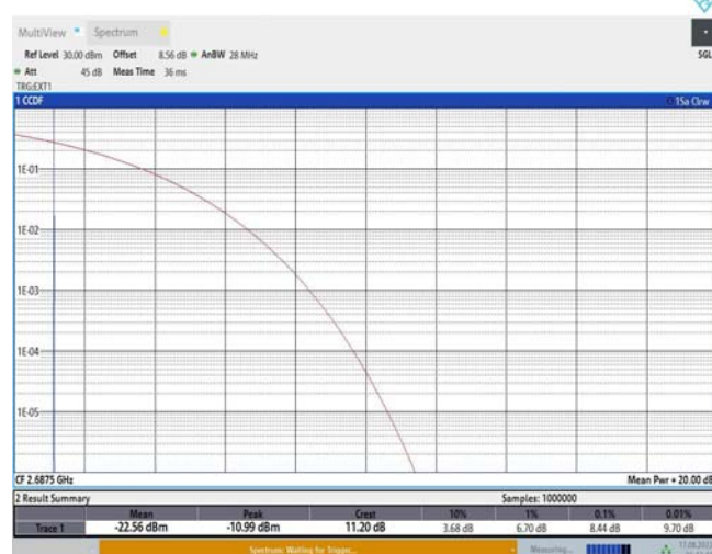
Band41-5MHz-QPSK-41565-25RB#0
