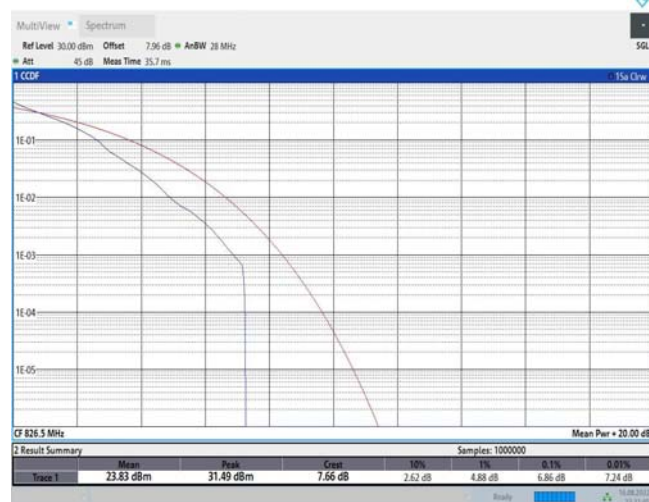
Band26-5MHz-QPSK-26815-25RB#0
