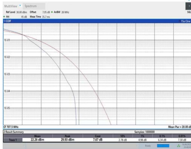
Band12-5MHz-16QAM-23095-25RB#0
