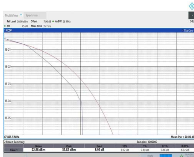
Band26-3MHz-16QAM-26915-1RB#0
