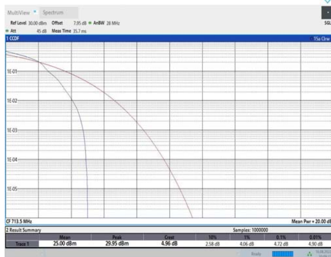
Band12-5MHz-16QAM-23155-25RB#0
