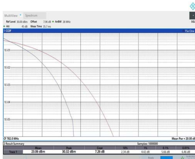
Band13-10MHz-16QAM-23230-1RB#0
