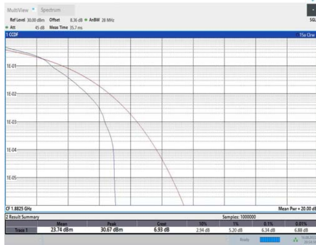
Band25-1.4MHz-16QAM-26365-6RB#0
