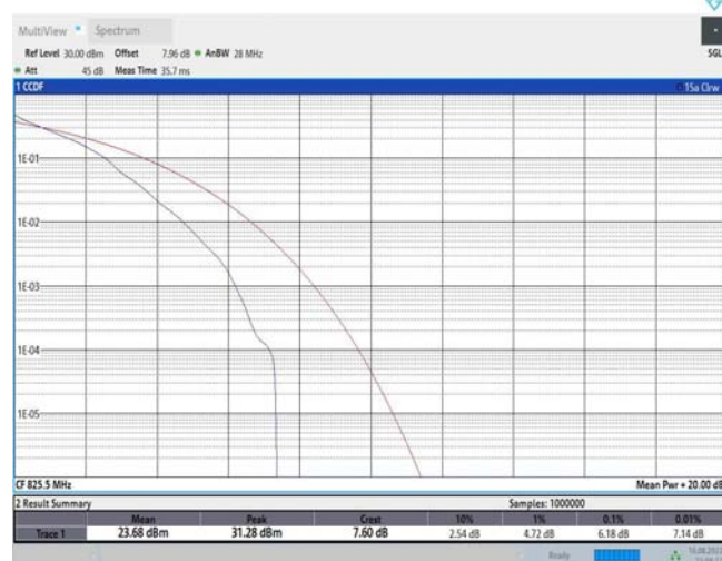
Band26-3MHz-QPSK-26805-15RB#0
