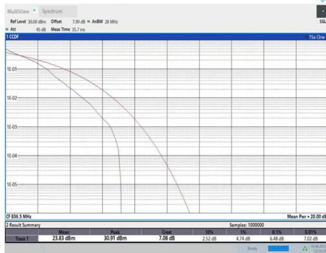
Band26-1.4MHz-QPSK-26915-6RB#0
