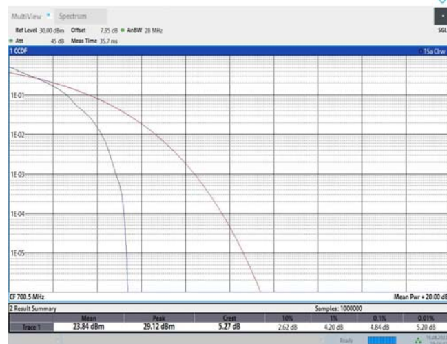
Band12-3MHz-QPSK-23025-15RB#0
