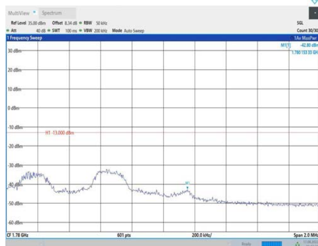
Band66-5MHz-16QAM-132647-1RB#24
