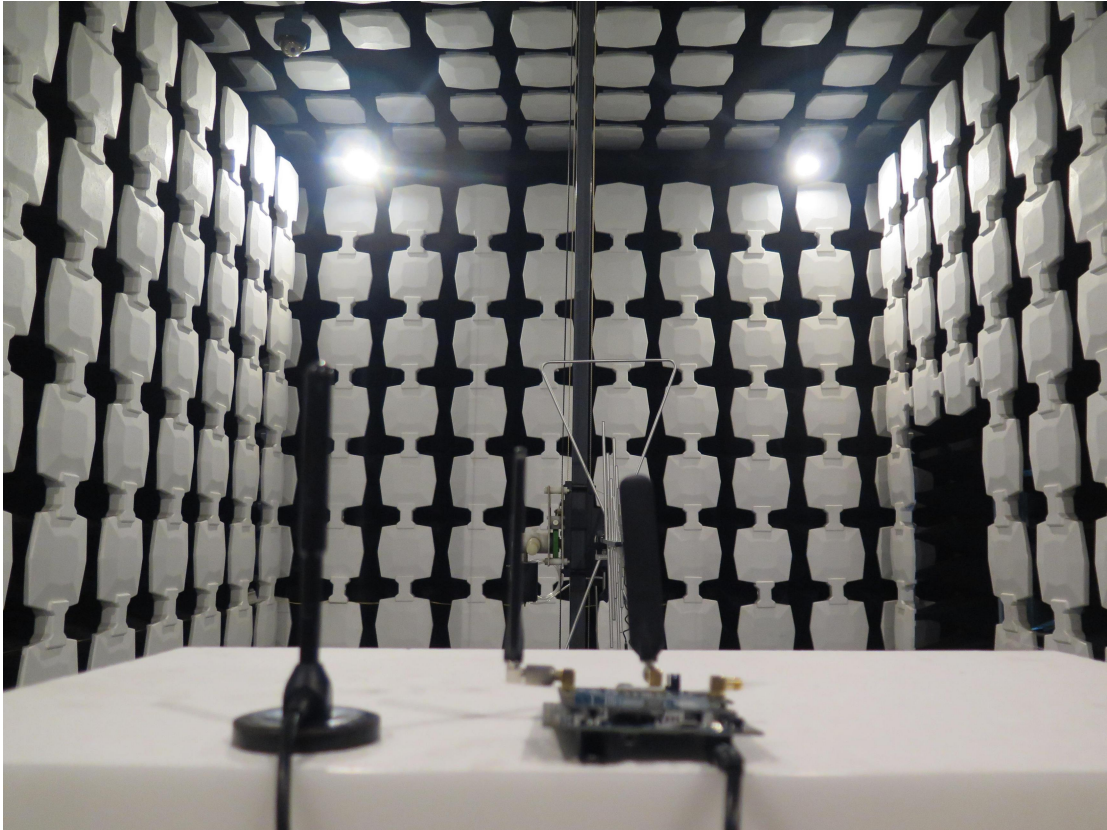
A7672SA RSE 30MHz-3GHz
