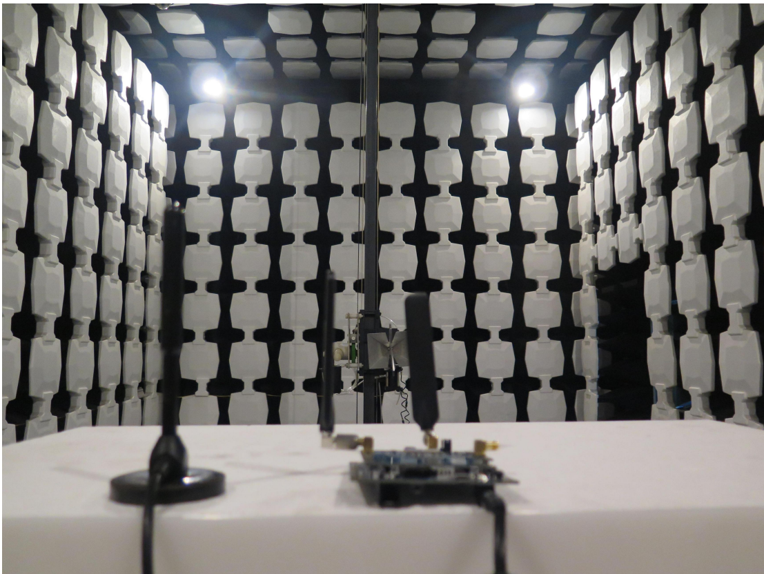
A7672SA RSE 3GHz-18GHz
