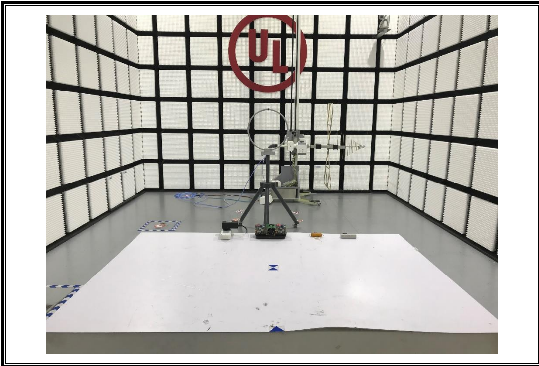
RADIATED EMISSIONS MEASUREMENT SETUP (Below 30MHz)
