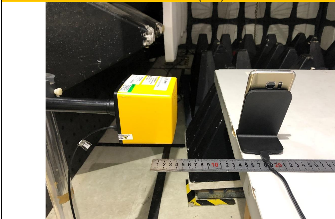
E-Field Strength and H-Field Strength Position B (15cm)
