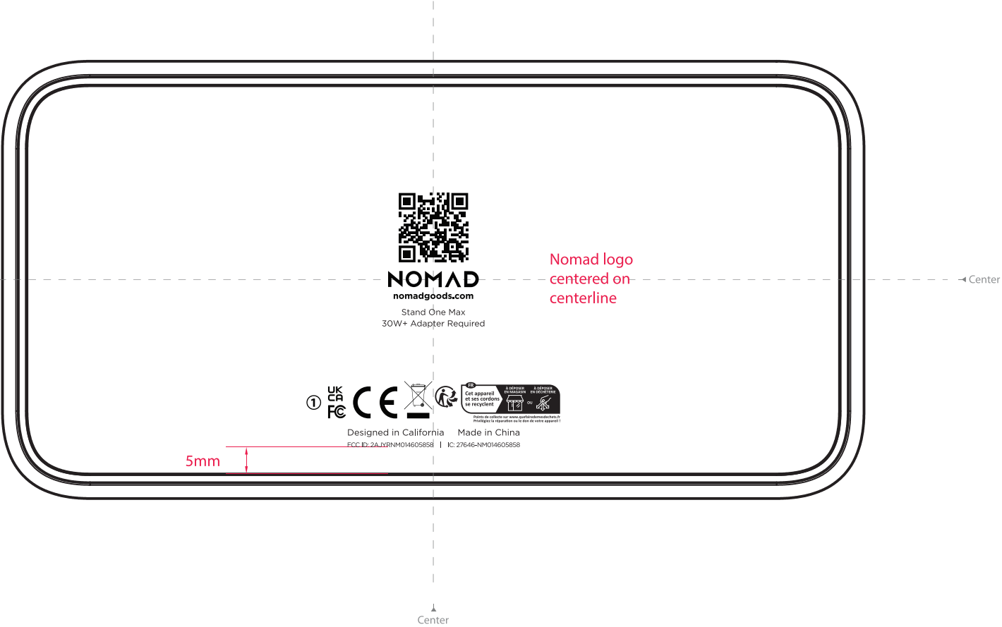
BOTTOM VIEW SCALE 1:1
