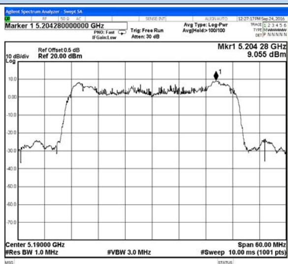
Chain 0-5190MHz
