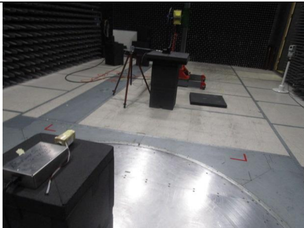
9kHz-30 MHz, Antenna Perpendicular
