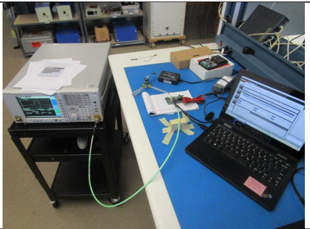
Conducted Bench
