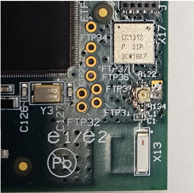
Note: U.FL connector was used for conducted measurements and is not part of the final product
