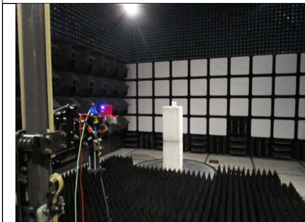
Above 1 GHz Radiated Emissions
