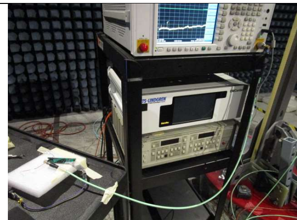
Conducted Measurements
