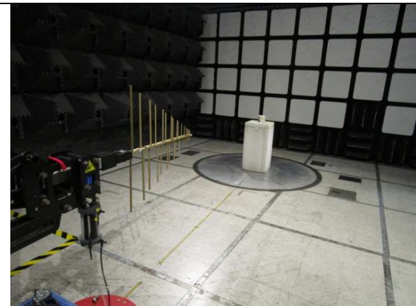
Below 1 GHz Radiated Emissions
