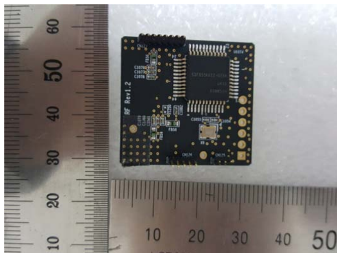
View of RF Board (Bottom)
