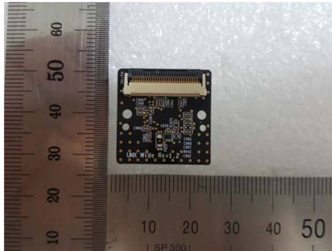
View of Wide Sensor Board (TOP)
