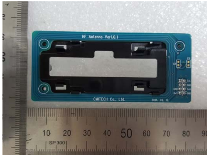
View of Antenna Board (TOP)
