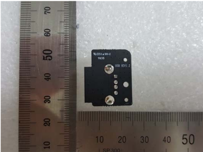
View of USB Board (Bottom)
