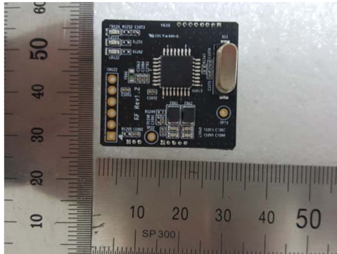
View of RF Board (TOP)
