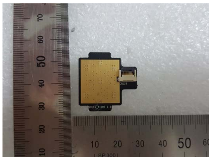
View of LED Board_ RIGHT (Bottom)
