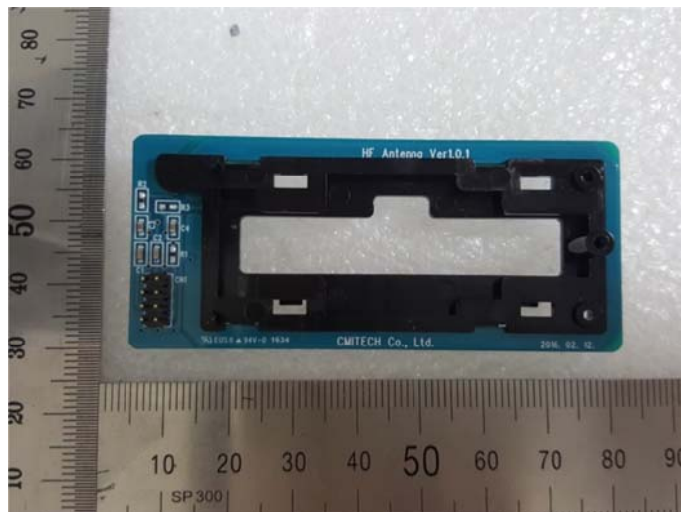
View of Antenna Board (Bottom)
