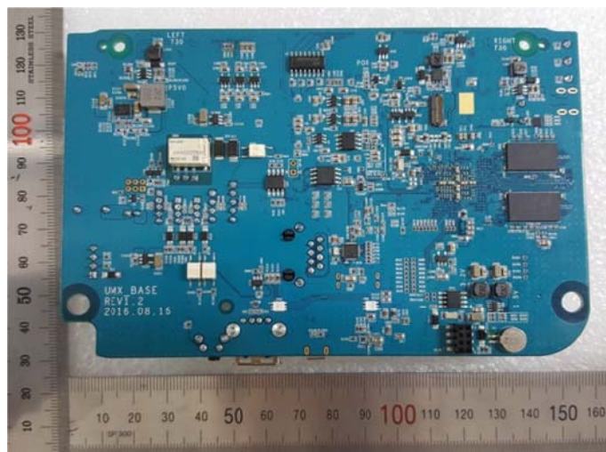
View of Main Board (Bottom)
