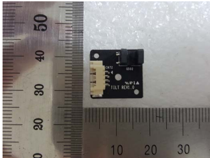
View of TILT Sensor Board (TOP)
