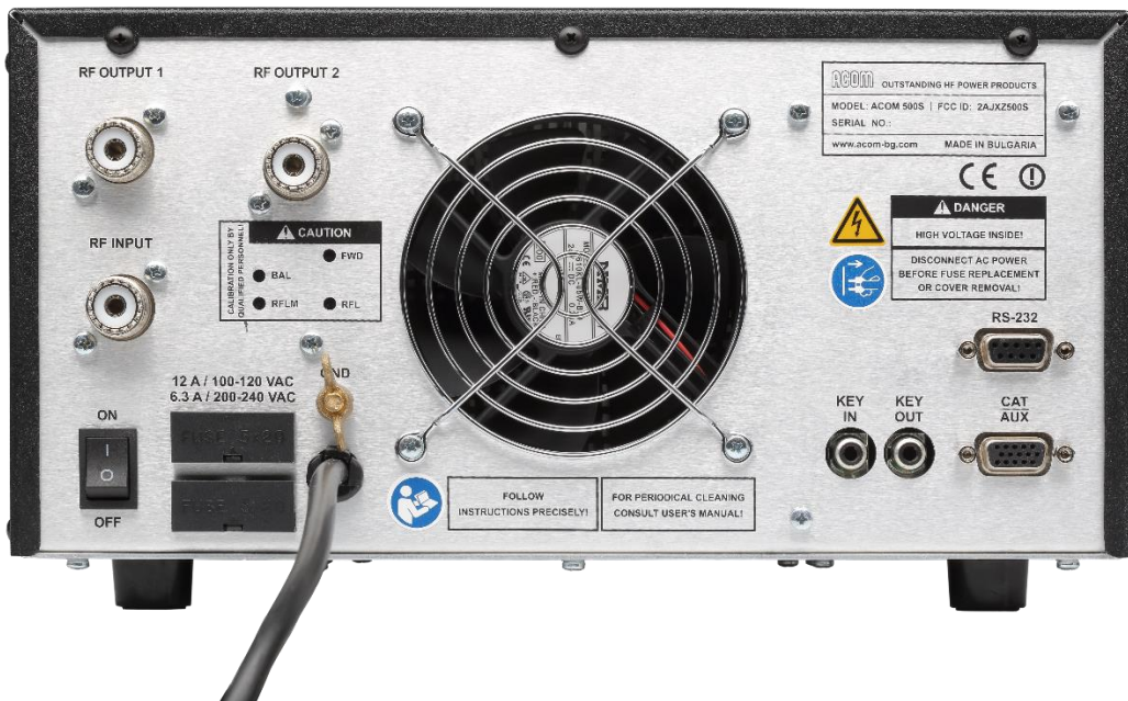
Figure 2- Rear view
