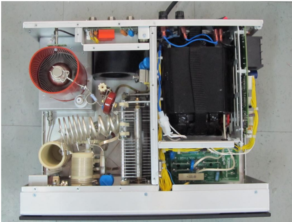
Fig.3 Top View
