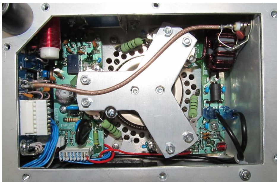
Fig.4 Bottom View – Tube Deck (screen cover removed)
