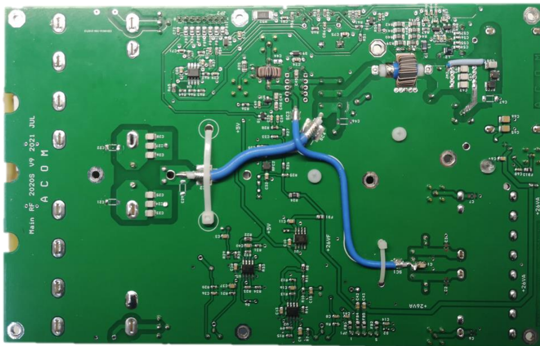
Figure 37 - Main-RF V9 top side
