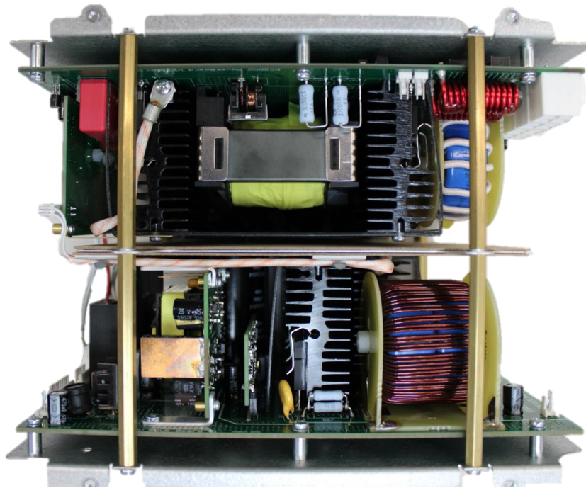
Figure 15 - Power supply bottom side
