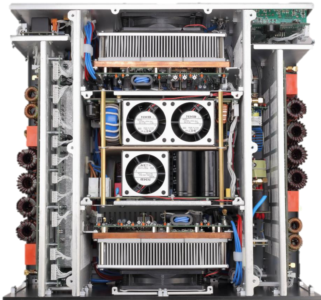
Figure 1 - ACOM 2020S top view
