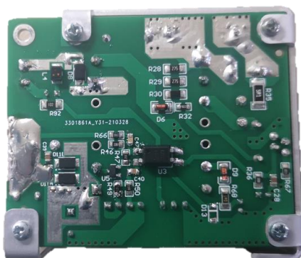
Figure 22 - Aux_Supply_V1 bottom side
