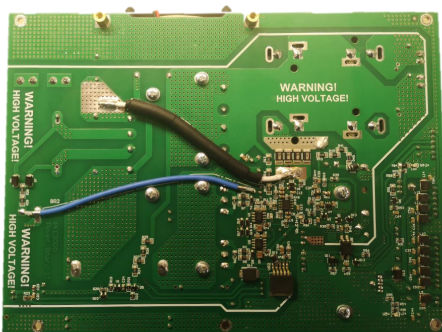
Figure 17- PFC3000_PWRB_V1 top side
