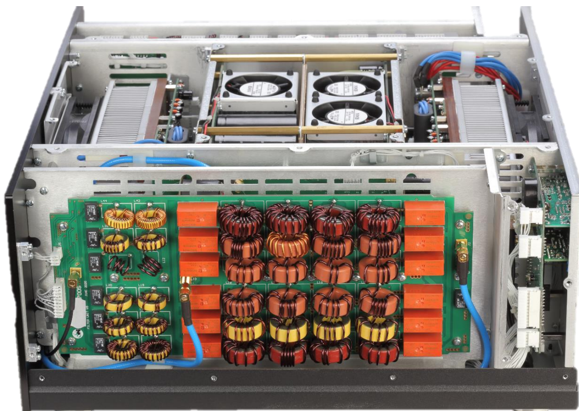
Figure 2 - ACOM 2020S side view
