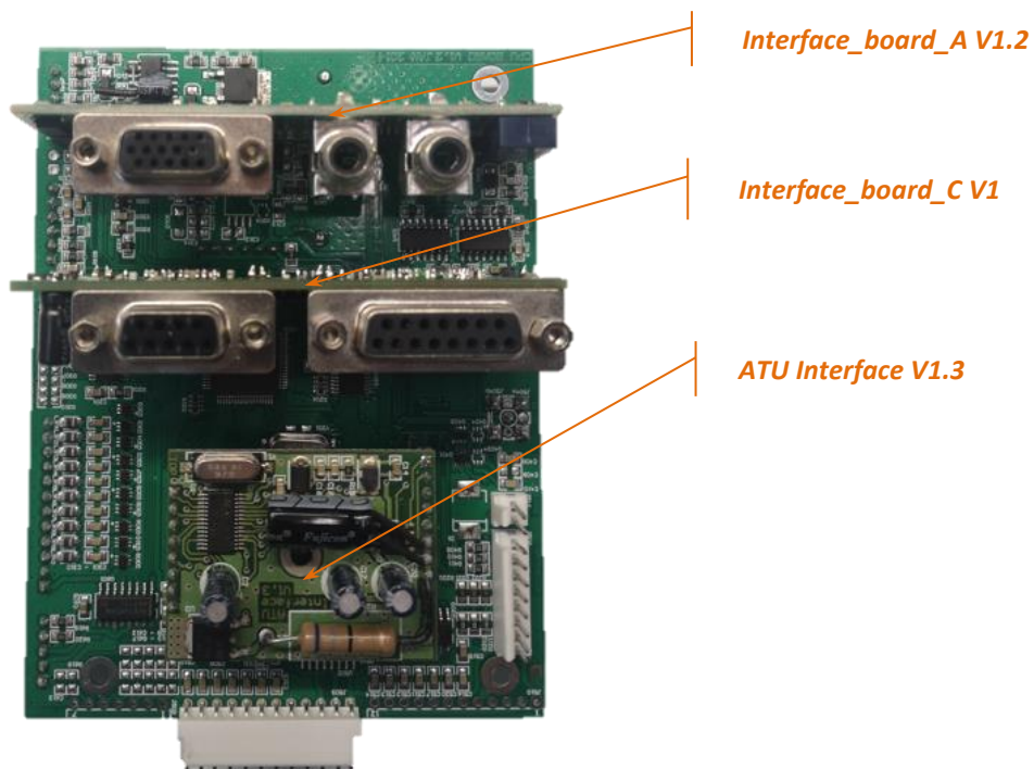
Figure 35 - CPU top side
