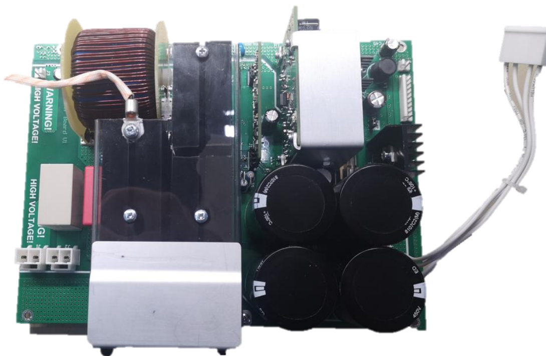
Figure 17- PFC3000_PWRB_V1 top side
