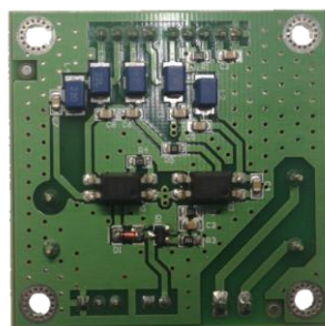
Figure 30 - Standby_PS3000_V1 bottom side
