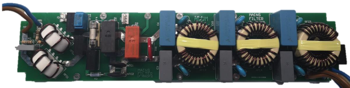
Figure 31 - Mains_filter_3kW_V7 top side
