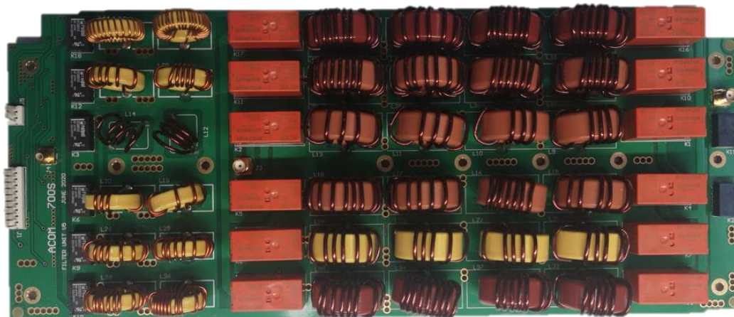
Figure 33 - A700S_Filter_Unit_V5 top side
