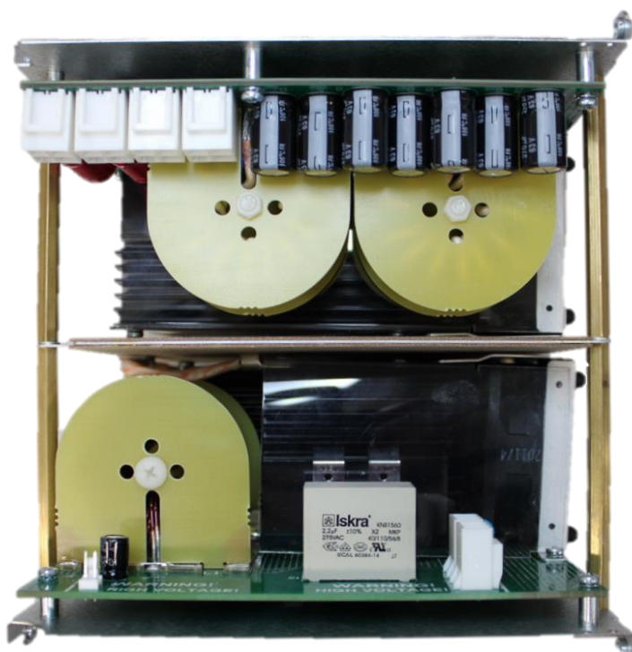
Figure 13 - Power supply top side
