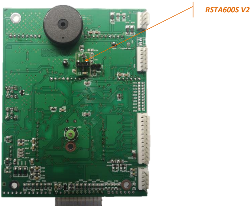
Figure 36 - CPU bottom side
