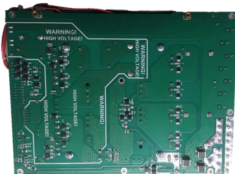
Figure 23 -DC3000_PWRB_V1 top side
