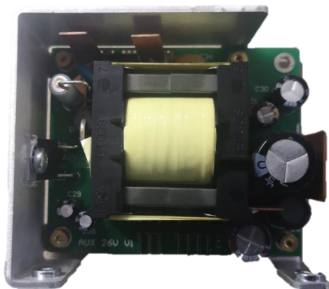
Figure 21 - Aux_Supply_V1 top side
