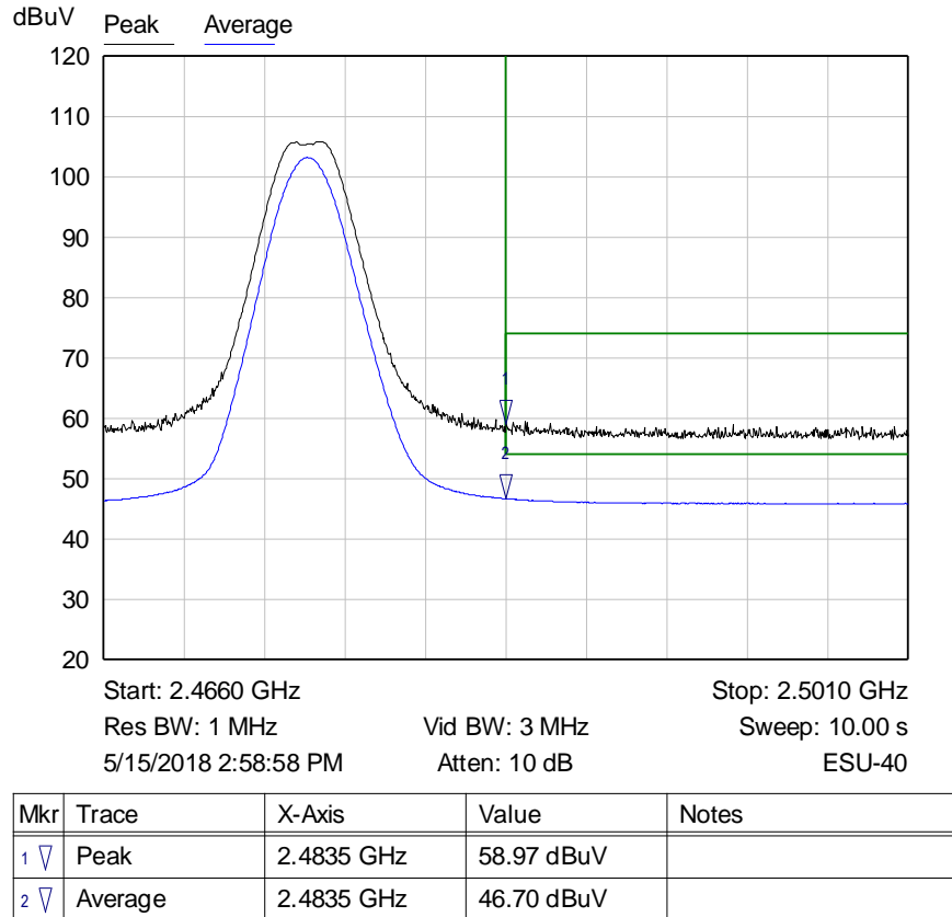
Graph 10: Radiated Upper Band Edge Plot
