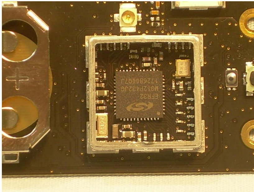
Photograph 9 – View of the Circuitry Under the RF Shield
