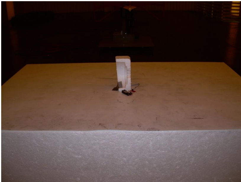
Photograph 2: Back View Radiated Emissions Configuration – 30 MHz to 1000 MHz
