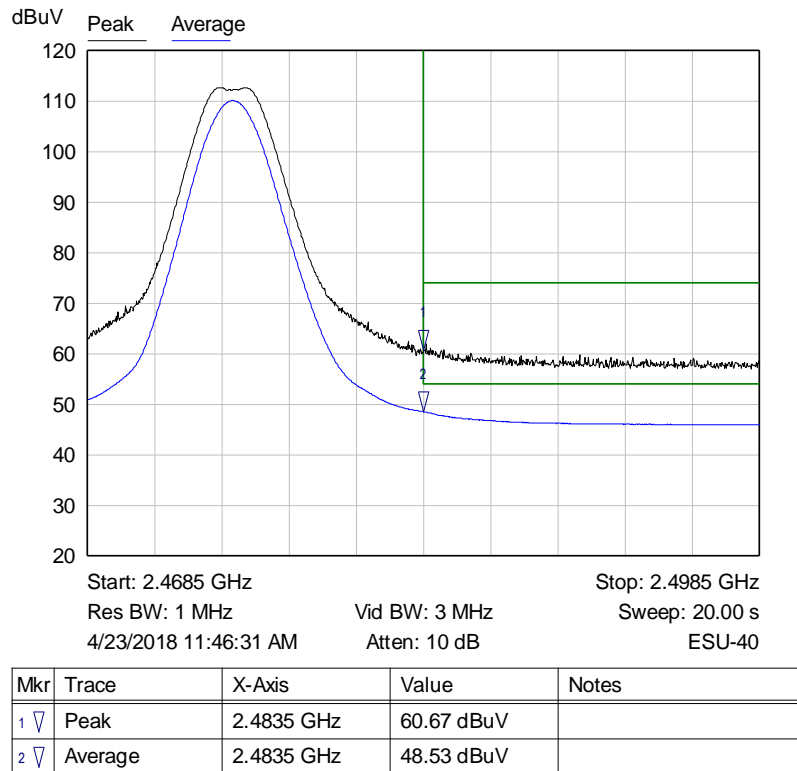
Graph 10: Radiated Upper Band Edge Plot
