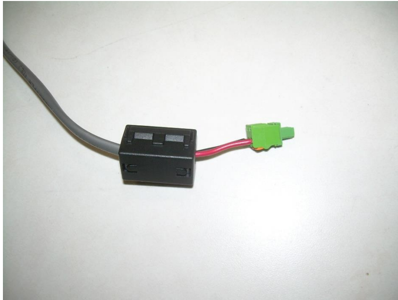
Photograph 15 – View of the Ferrite Placement on the EUT Power Cable
