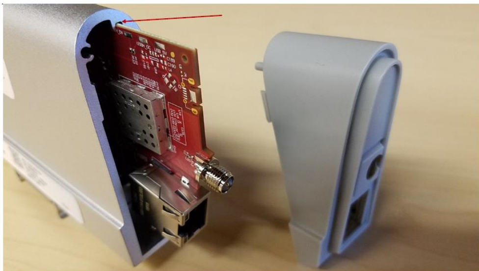
Photograph 5 - PCB Entry and Mounting
