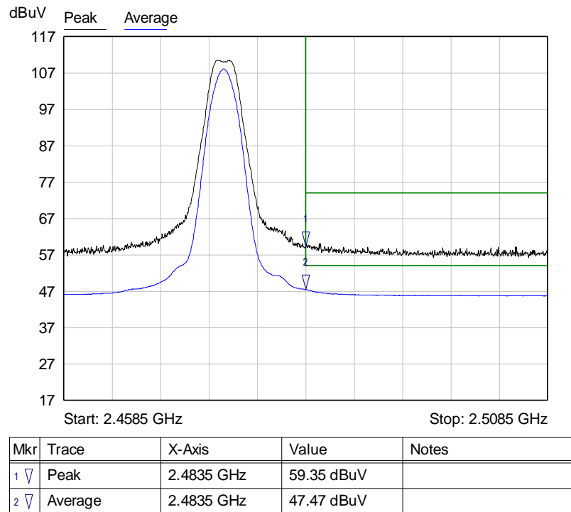
Graph 8: Radiated Upper Band Edge Plot
