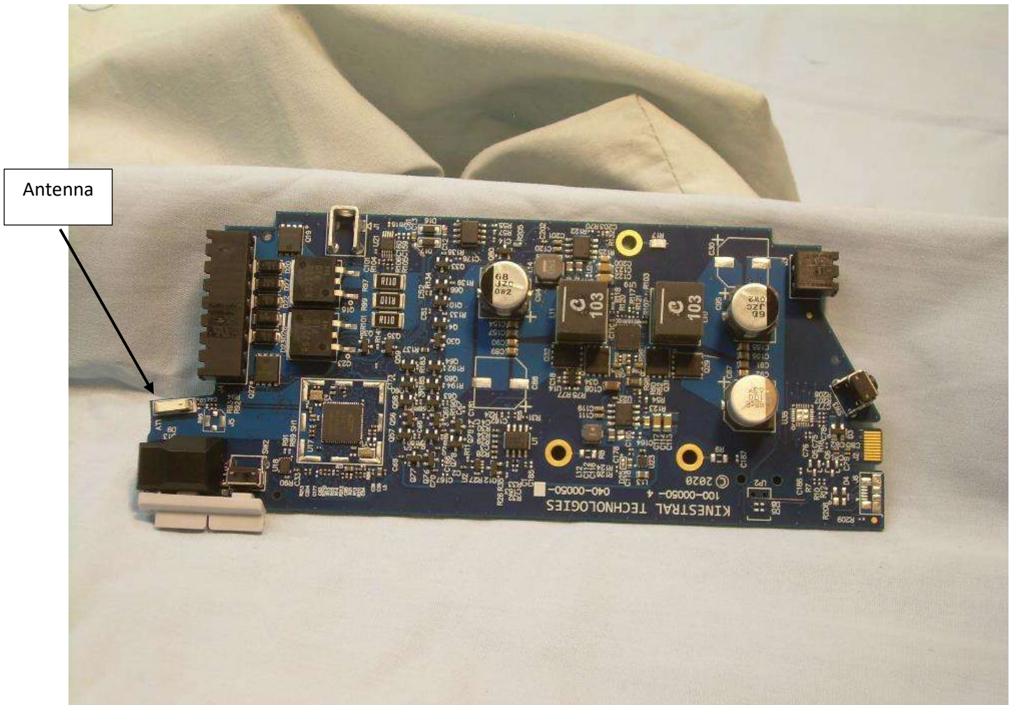
Photograph 2 – Top View of the PCB with Heatsink Removed
