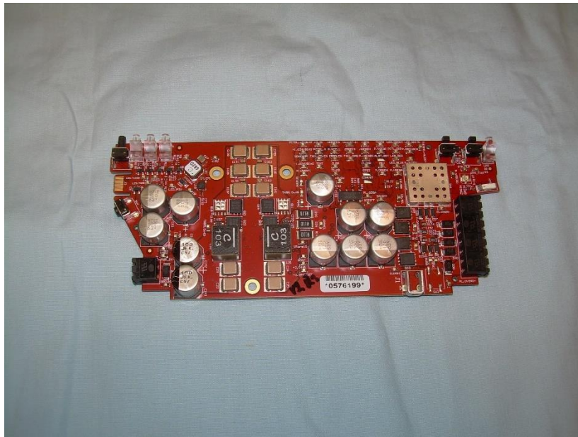
Photograph 11 - View of the Top Side of the PCB
