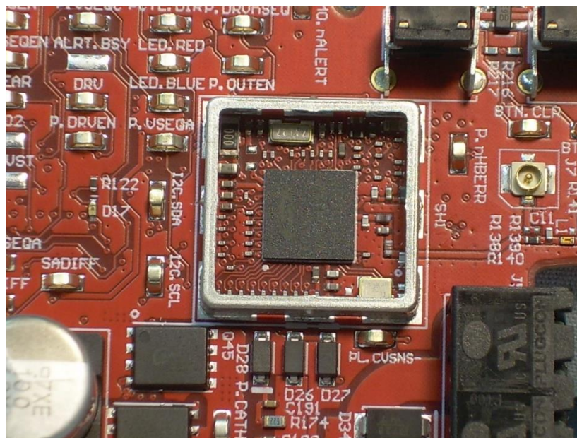
Photograph 12 - View of the Circuitry Under the RF Shield
