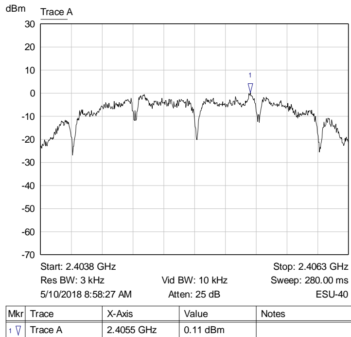
Graph 11: Lowest Channel 3 kHz PSD Plot
