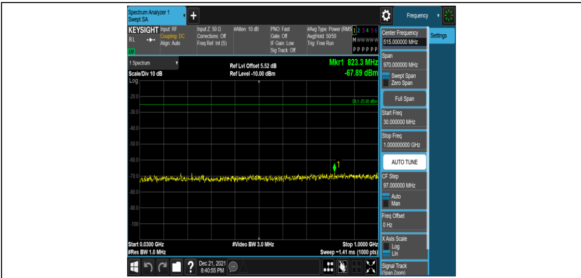
Band7-5MHz-QPSK-20775-1RB#0-Range3:30~1000MHz
