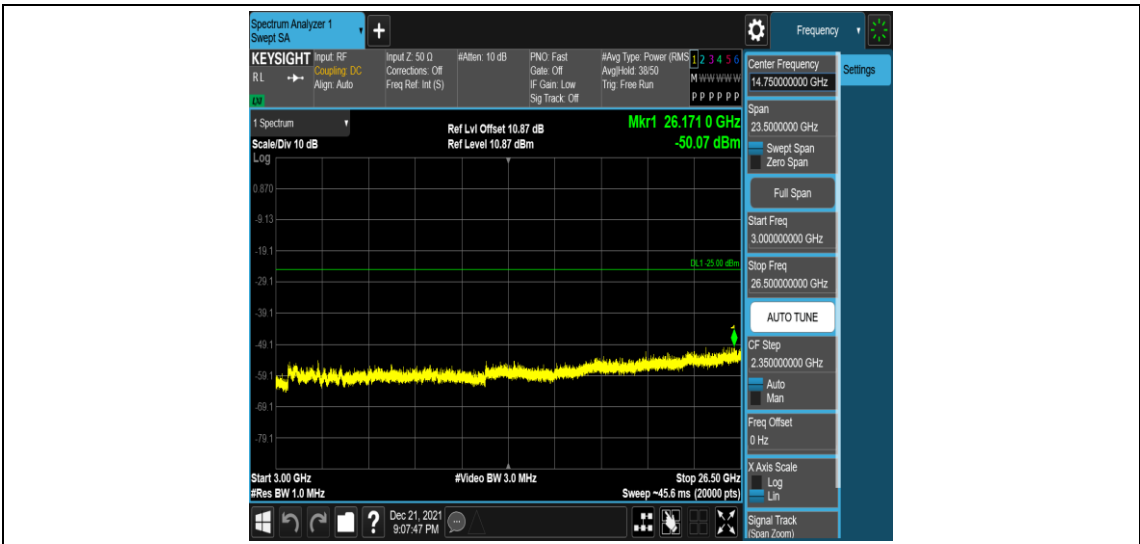
Band7-10MHz-QPSK-21400-1RB#0-Range5:3000~26500MHz
