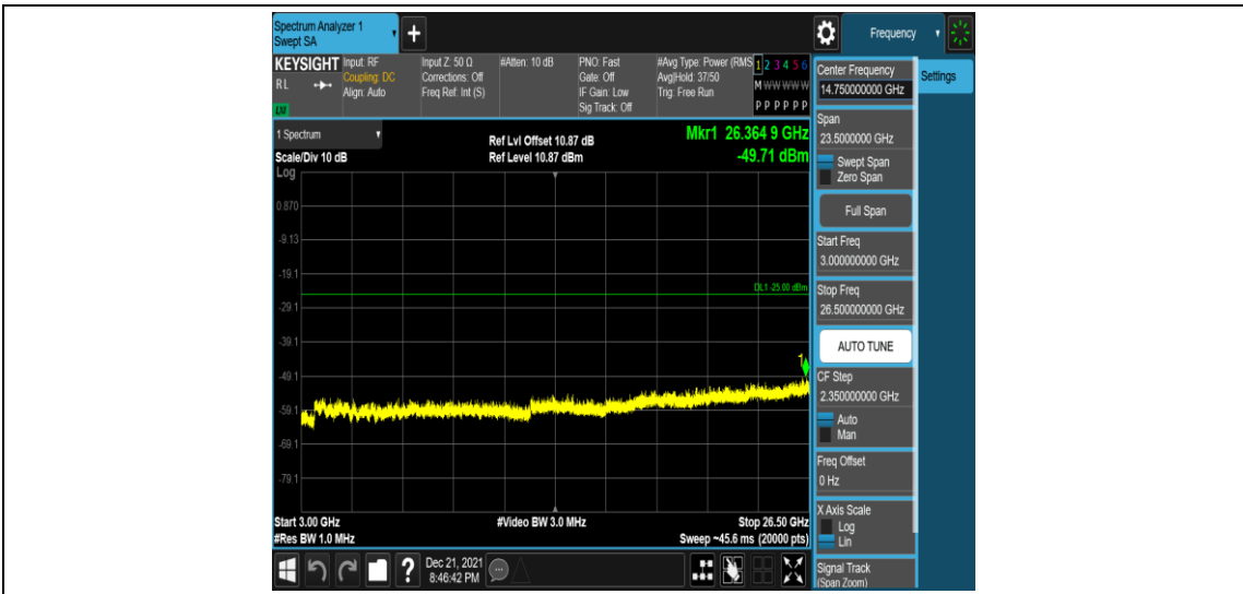
Band7-5MHz-16QAM-21425-1RB#0-Range5:3000~26500MHz
