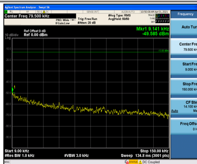
Band71_10MHz_16QAM_133172_1RB#0
