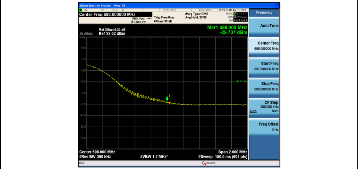
Band71_20MHz_16QAM_133222_1RB#0
