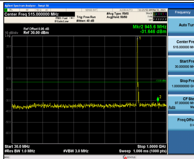
Band26-5MHz-16QAM-26740-1RB#0-Range4:1000~26500MHz
