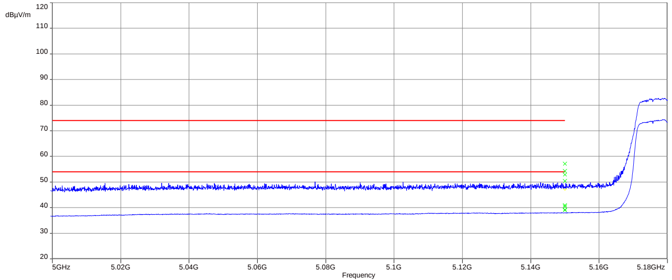
Plot 1: lower band edge; U-NII-1; lowest channel; a-mode/ nHT20-mode
