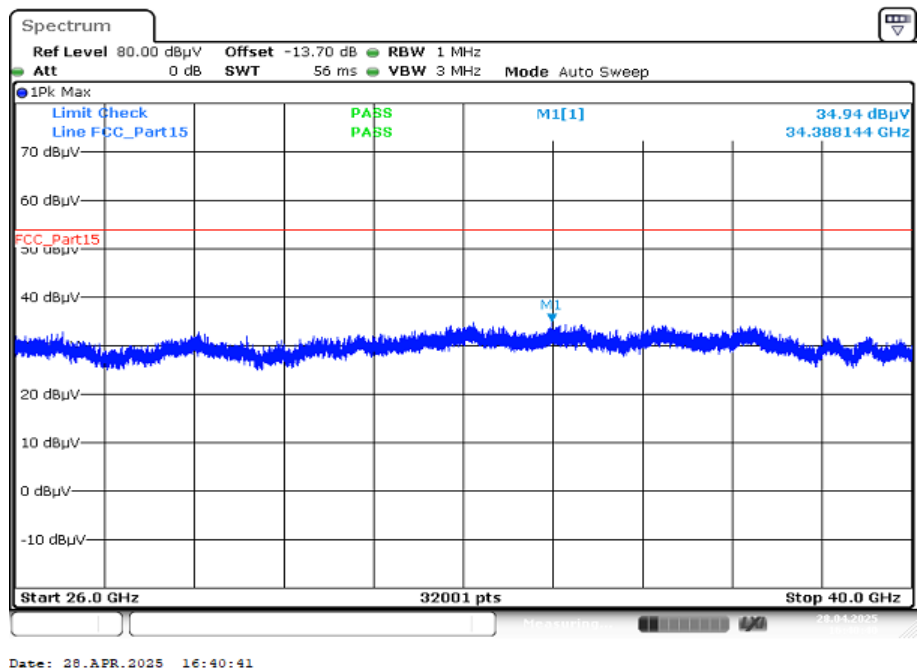
Plot 4: 26 GHz to 40 GHz; vertical & horizontal polarization; U-NII-1; valid for all channels and modes
