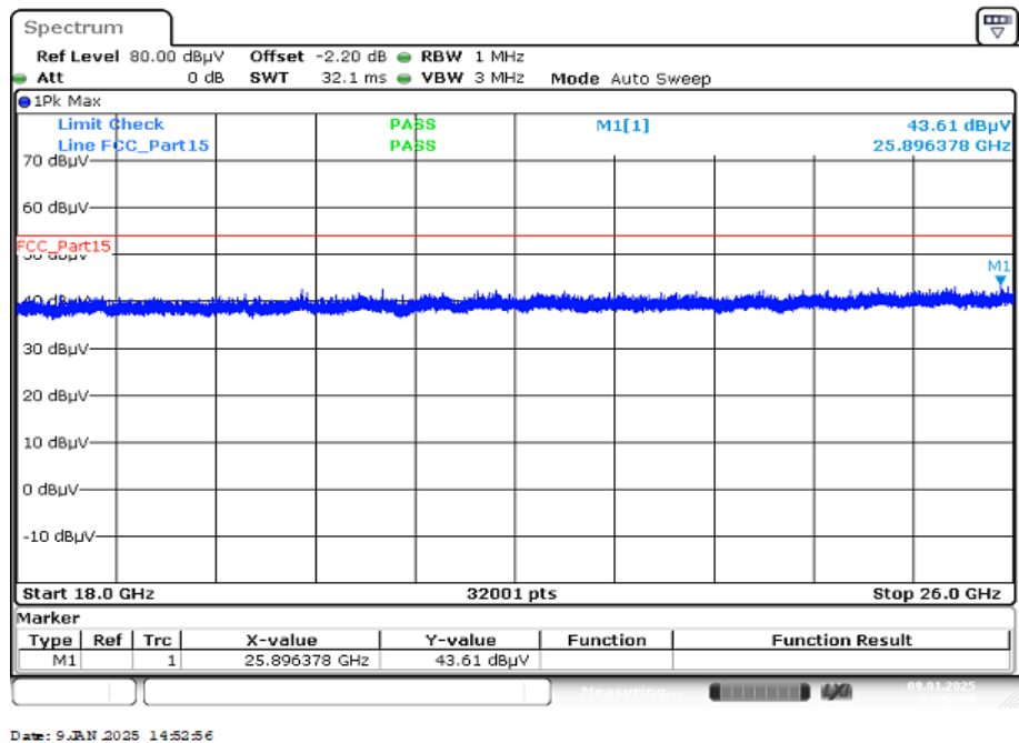
Plot 3: 18 GHz to 26 GHz; vertical & horizontal polarization; U-NII-1; valid for all channels and modes
