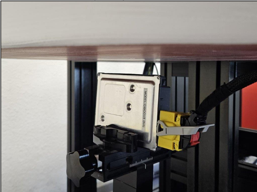
Photo 6: Test position right side with 20 mm distance
