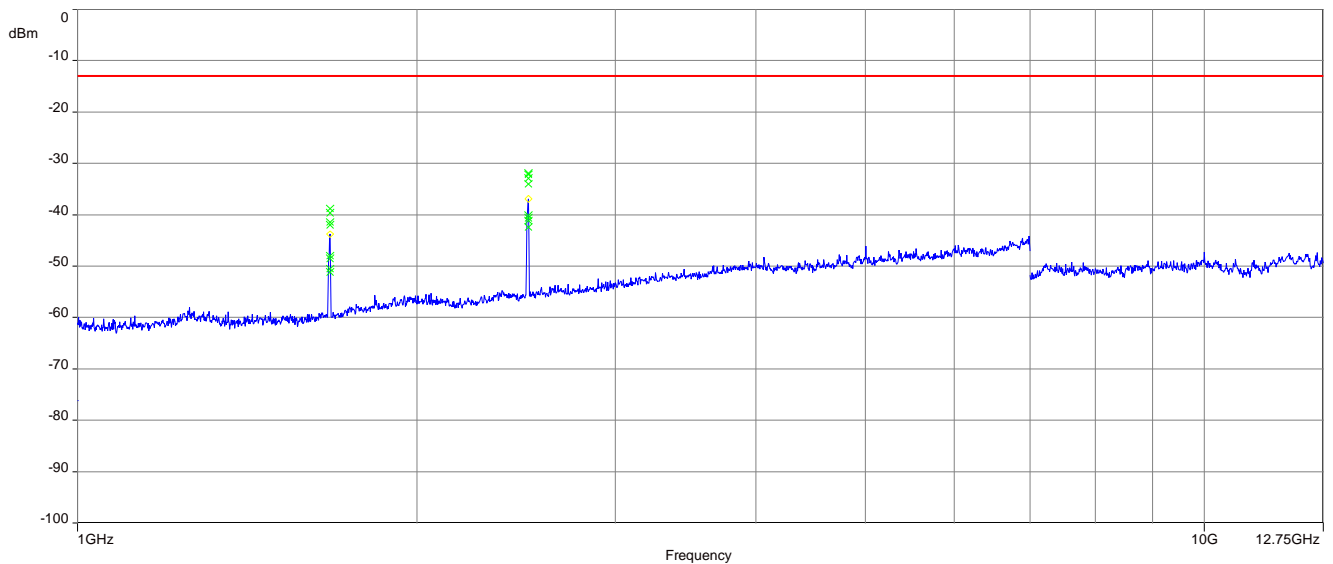
Plot 2: Channel 4180 (1 GHz – 12.75 GHz)
