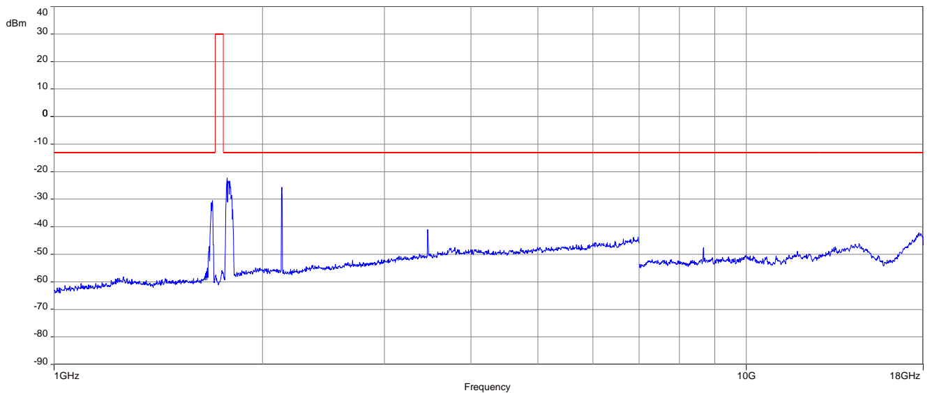
Plot 2: Channel 1412 (1 GHz – 18 GHz)
