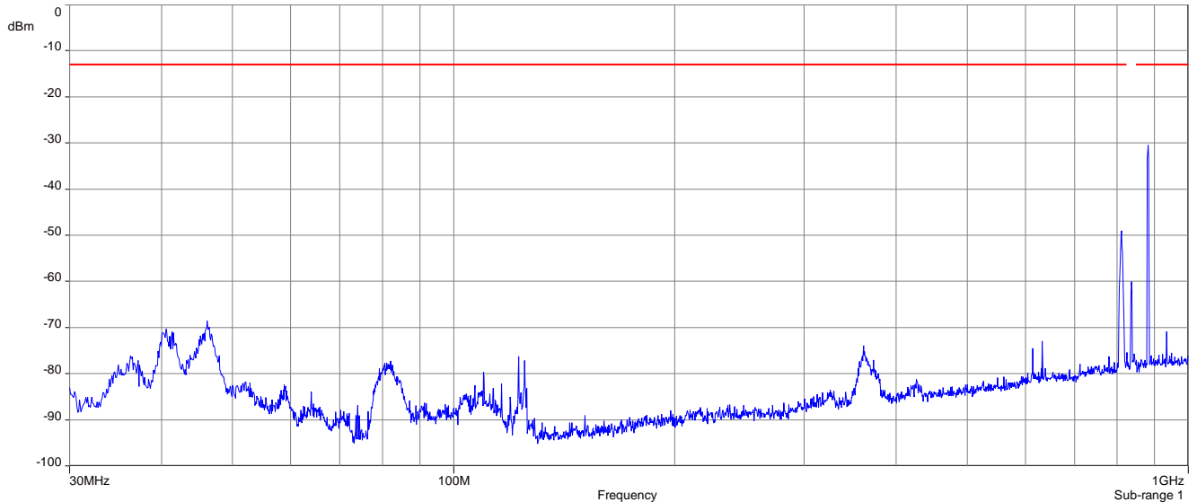
Plot 1: Channel 4180 (30 MHz – 1 GHz)
