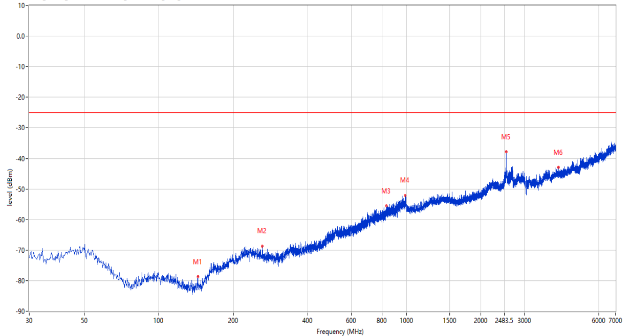
RSE Test case_CE FCC_FCC PART22&24&27_FCC PART 27_2535_LTE B7
