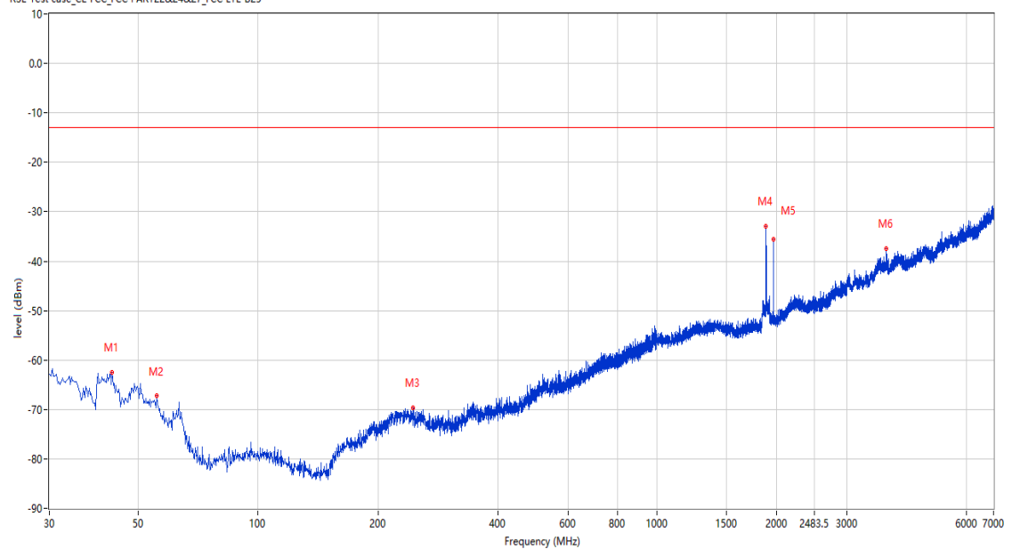
RSE Test case_CE FCC_FCC PART22&24&27_FCC LTE B25
