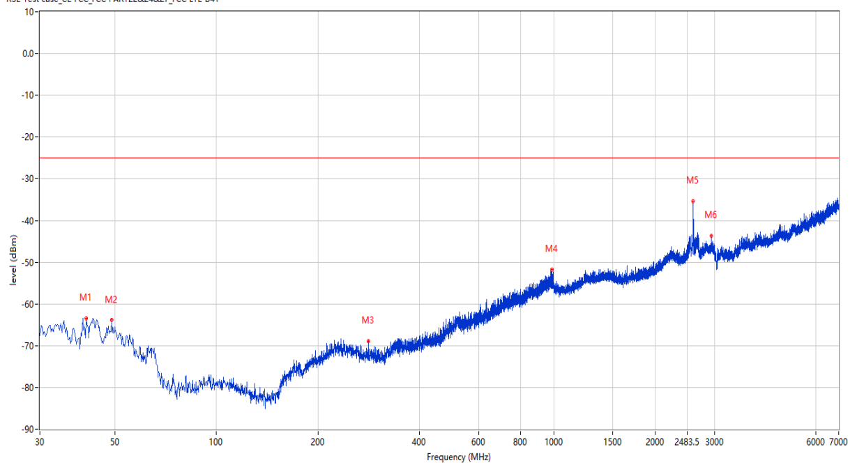
RSE Test case_CE FCC_FCC PART228&24&27_FCC LTE B41
