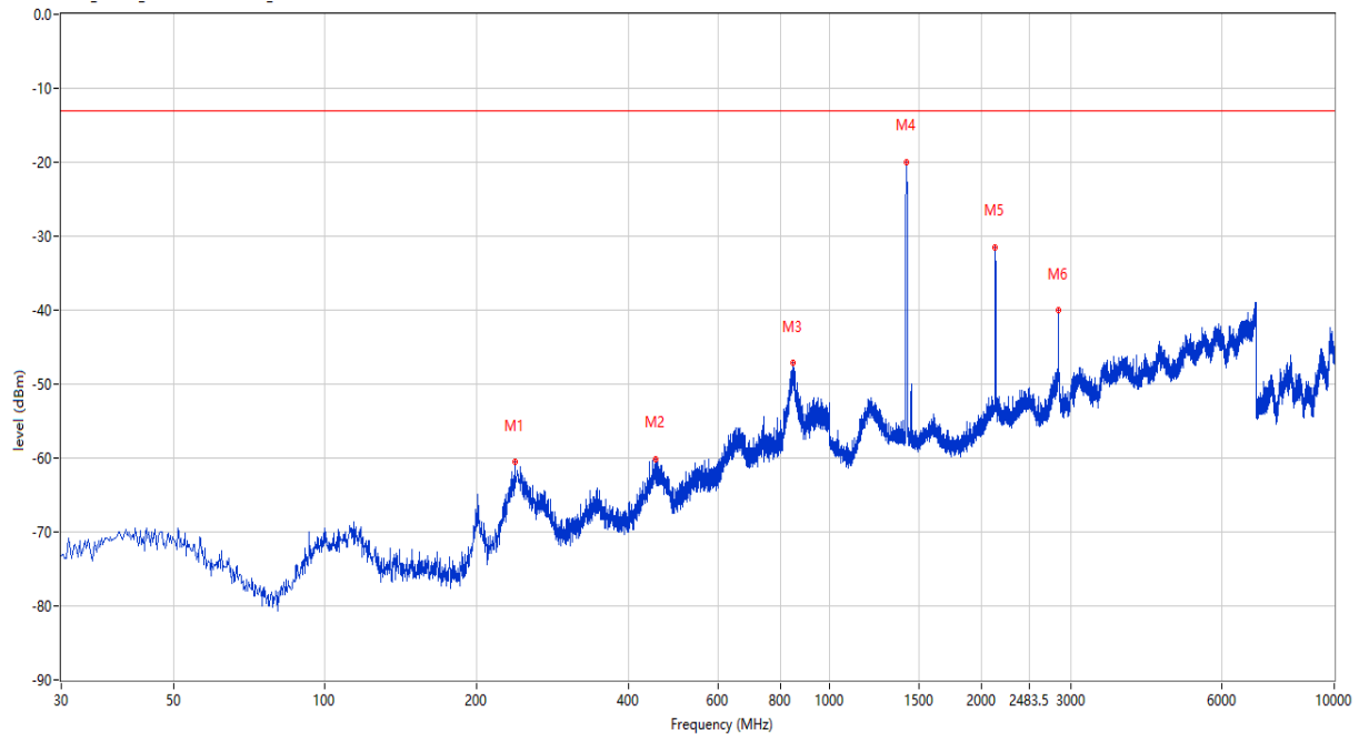
RSE Test case_CE_FCC_FCC PART228&248&27_FCC LTE B17
