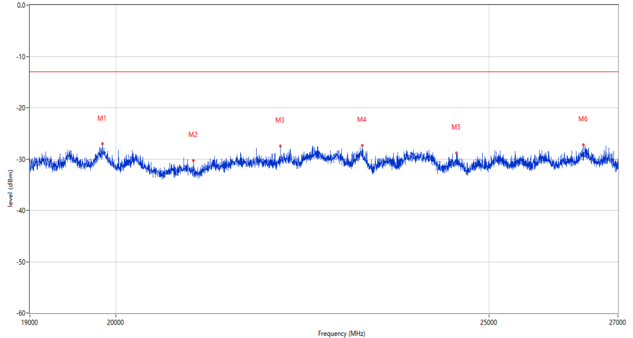
RSE Test case_CE FCC_FCC PART228&24&27_FCC GSM&CDMA&LTE&WCDMA 19-27G
