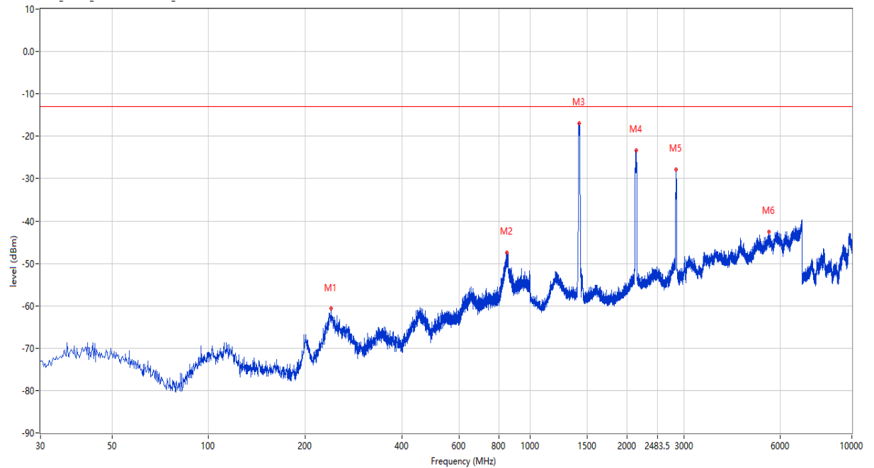
RSE Test case_CE_FCC_FCC PART22&24&27_FCC LTE B17
