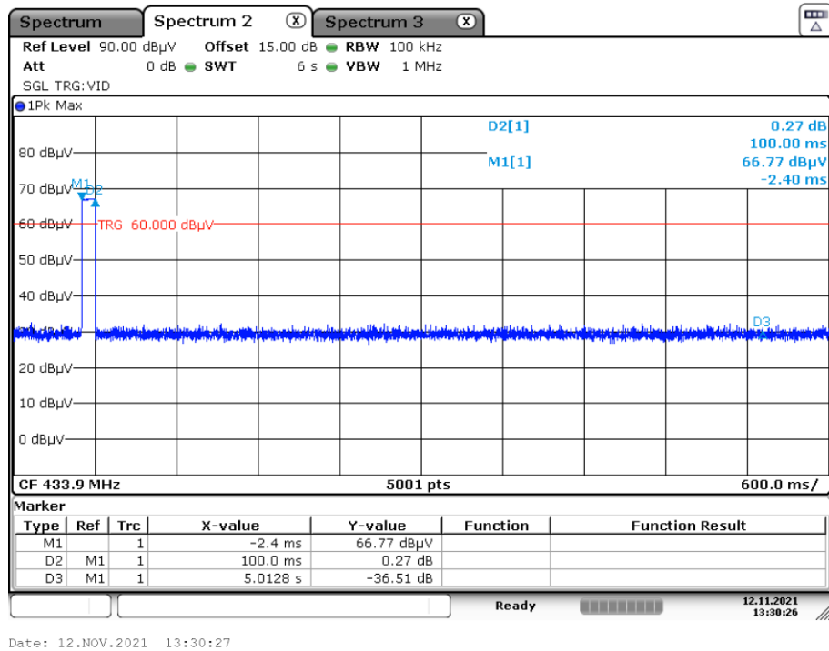
Plot 4: TX on time 433 MHz high duty cycle
