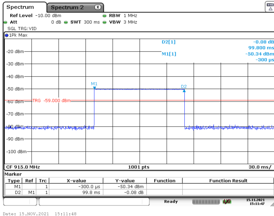
Plot 8: 915.0 MHz FSK max. frame length
