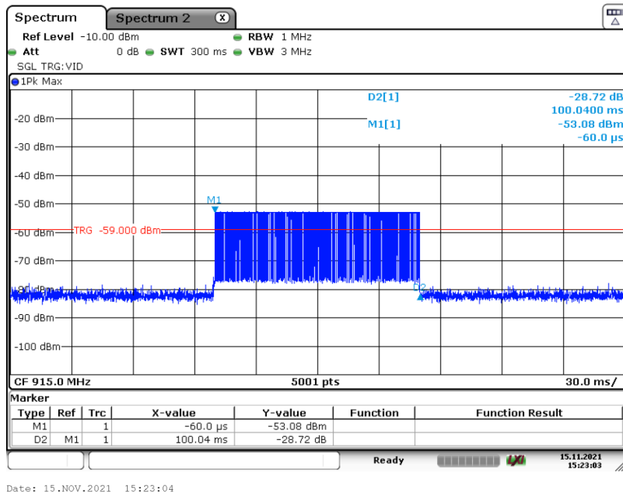
Plot 7: 915.0 MHz ASK max. frame length
