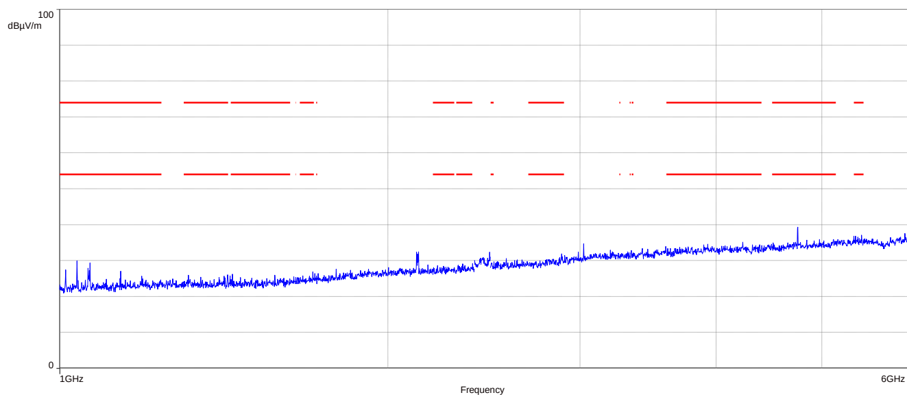
Plot 3: TX@431.9MHz, ASK, 1000 MHz to 6000 MHz, vertical & horizontal polarisation
