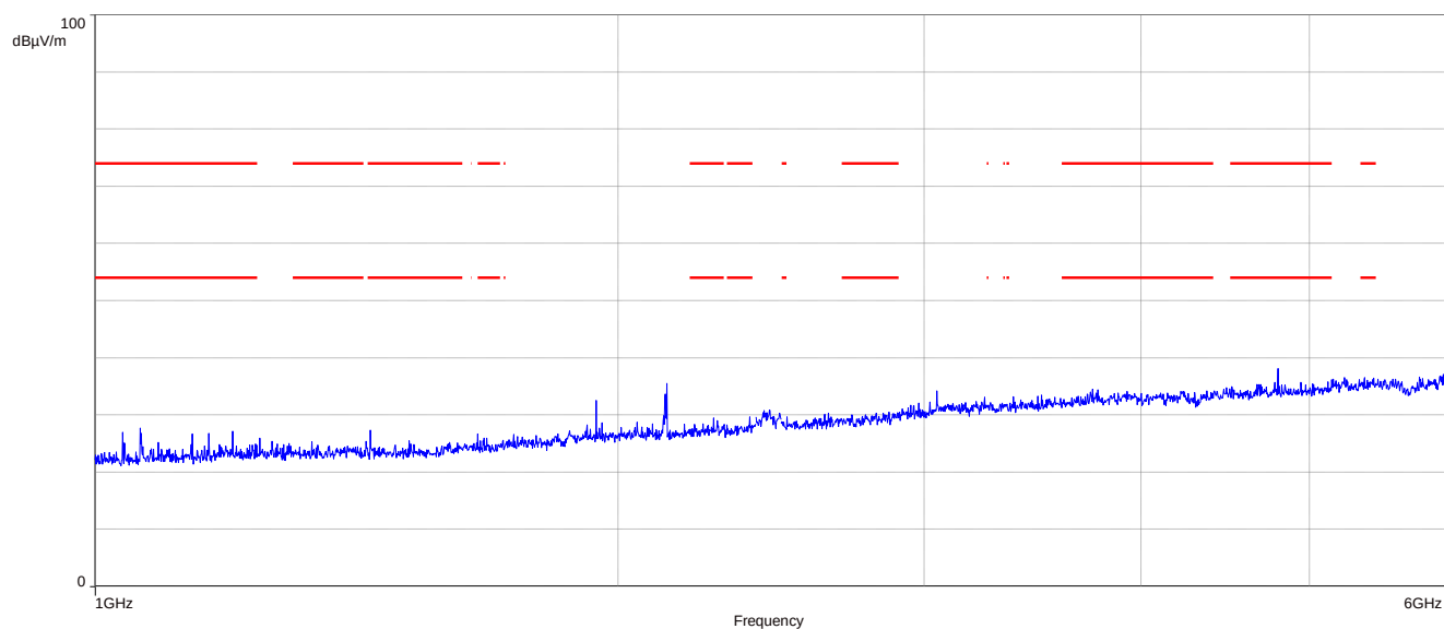
Plot 3: TX@435.9MHz, ASK, 1000 MHz to 6000 MHz, vertical & horizontal polarisation
