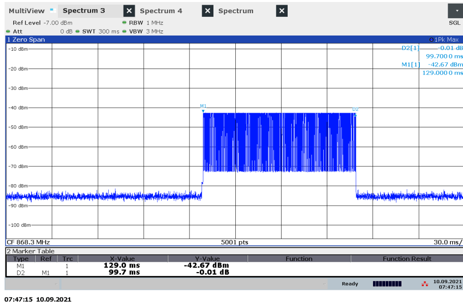
Plot 5: 868.3 MHz ASK max. frame length
