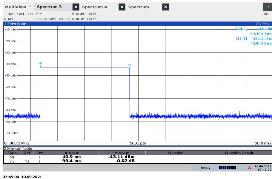
Plot 6: 868.3 MHz FSK max. frame length
