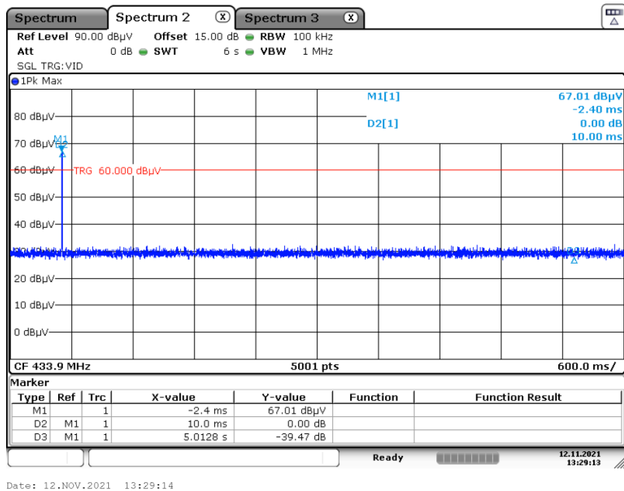
Plot 3: TX on time 433 MHz low duty cycle
