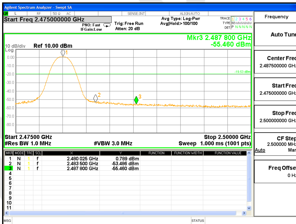
GFSK mode -- Highest
