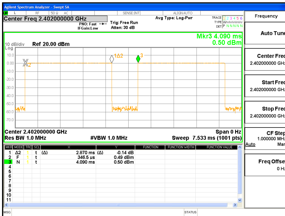
Test Mode: GFSK ---DH5
