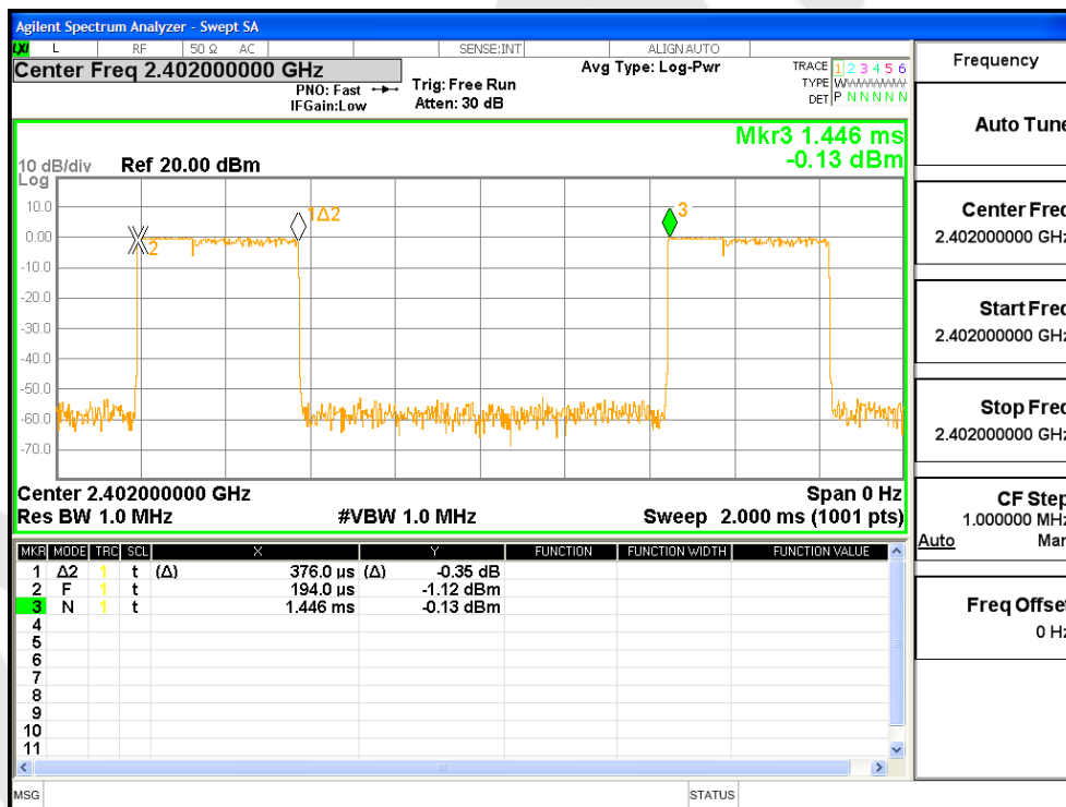
Test Mode: \pi/4 DQPSK ---2DH1
