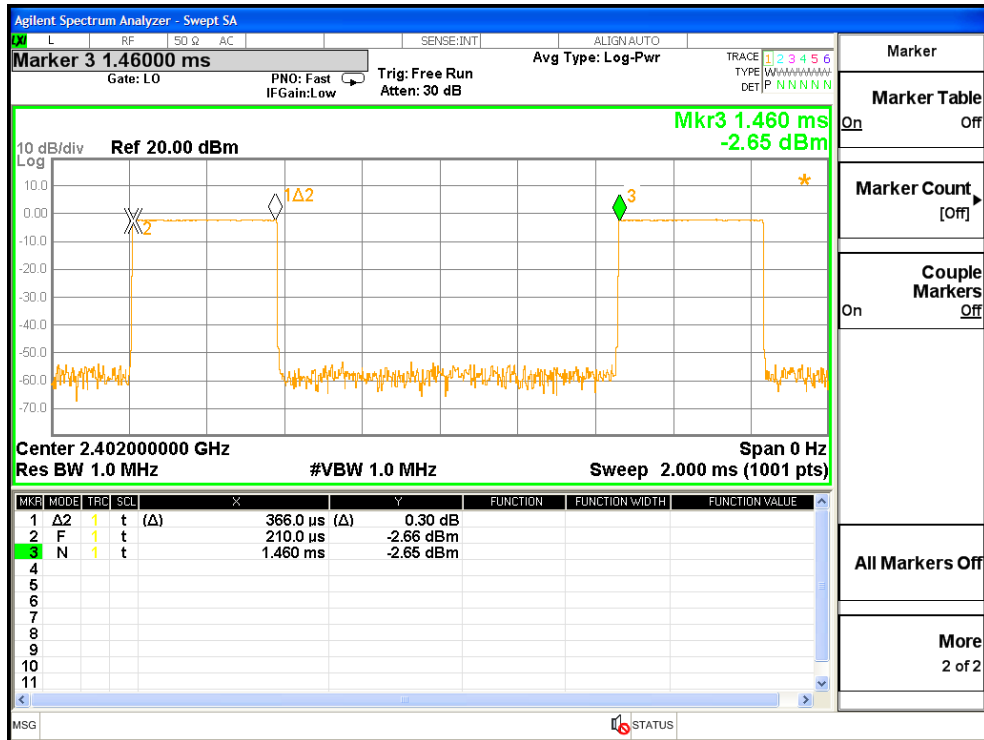
Test Mode: 8 DPSK ---3DH1
