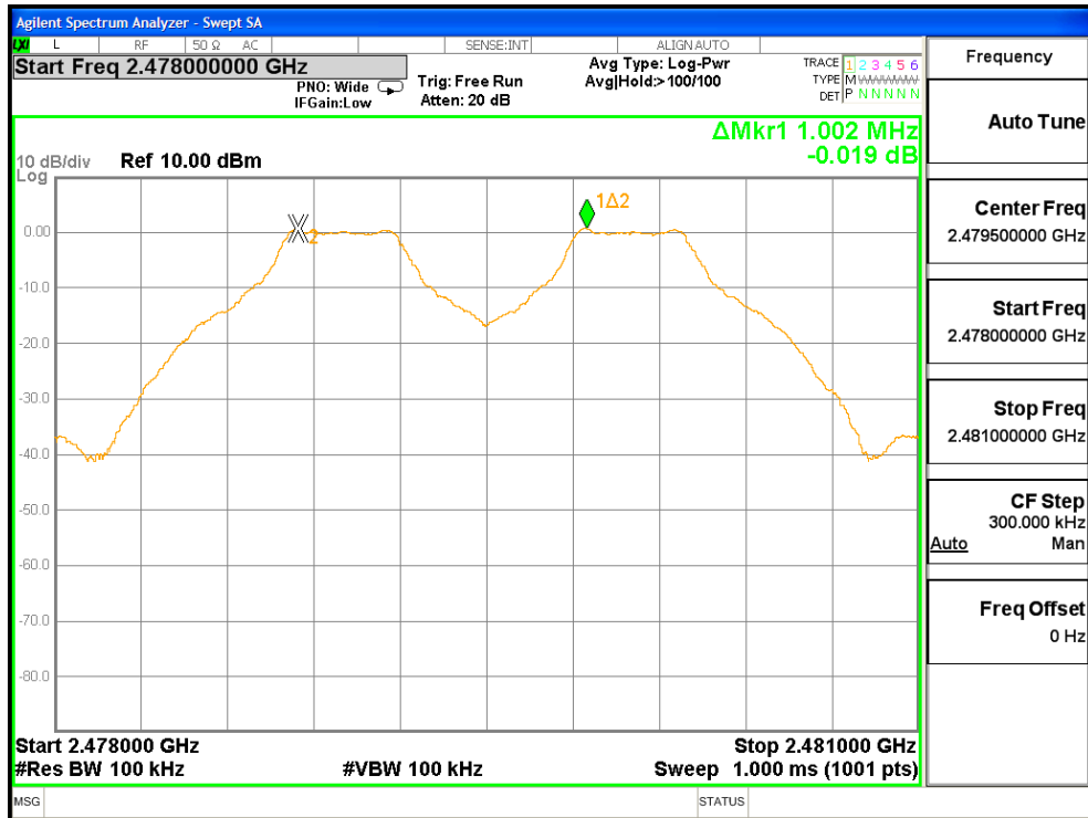
Test Mode: GFSK---High
