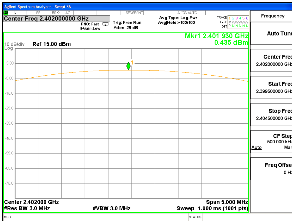
Test Mode: GFSK---Low
