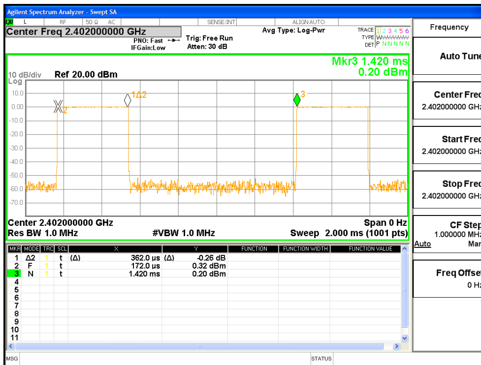
Test Mode: GFSK ---DH1
