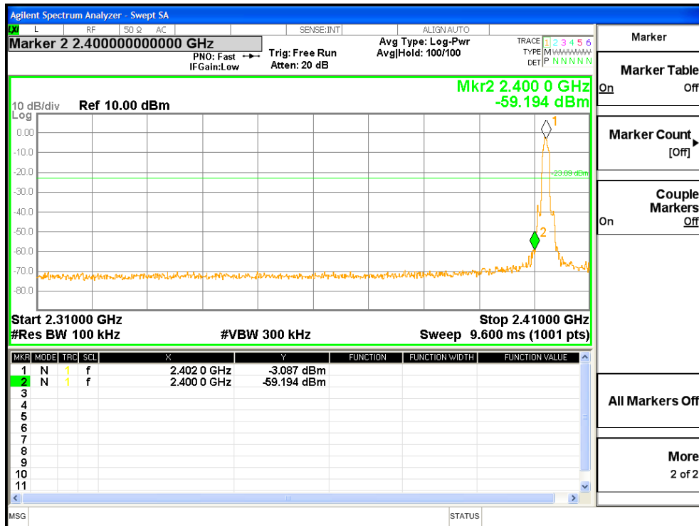
8DPSK mode -- Lowest
