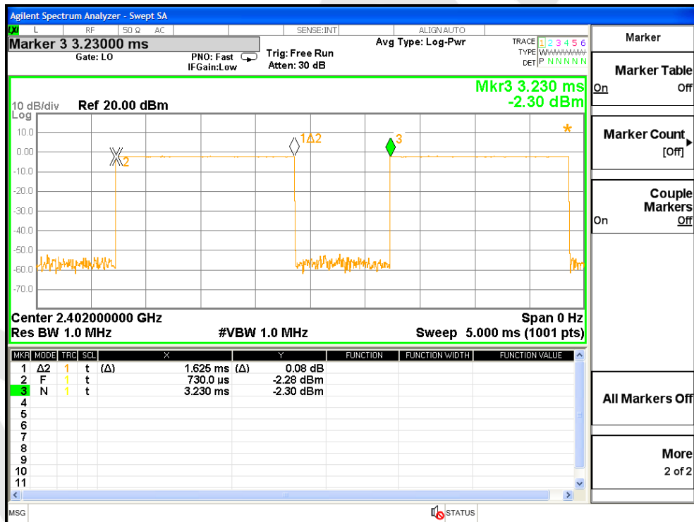
Test Mode: 8 DPSK ---3DH3
