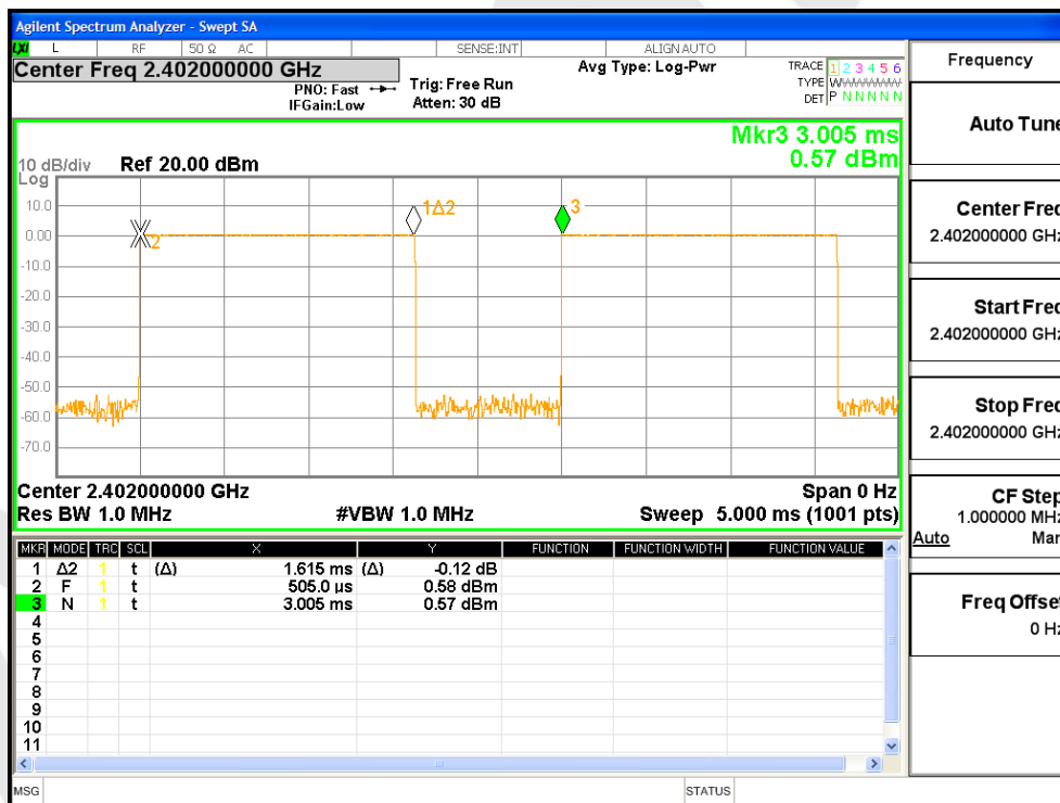
Test Mode: GFSK ---DH3
