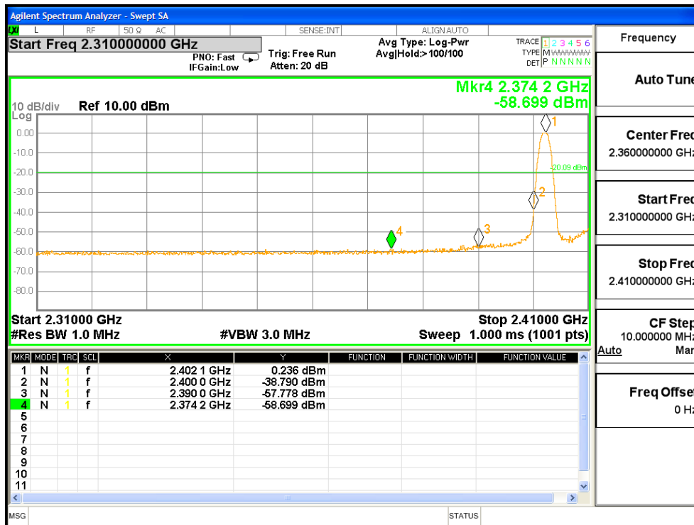
GFSK mode -- Lowest
