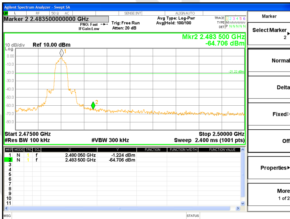
8DPSK mode -- Highest
