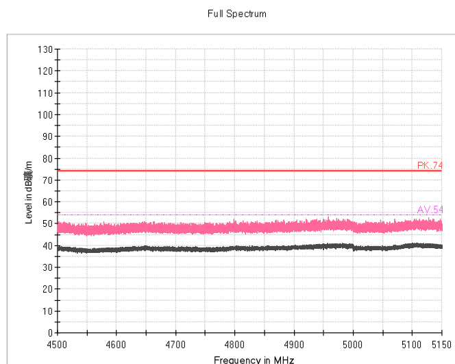
Radiated Emission Band Edge Channel No.:36 Test Mode: 802.11a Polarization: V
