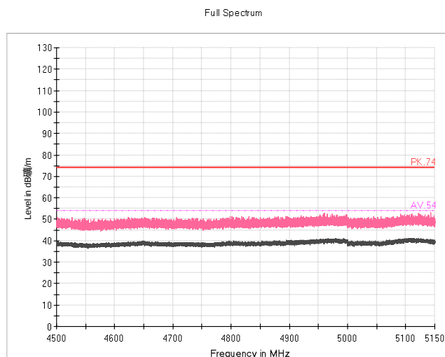
Radiated Emission Band Edge Channel No.:36 Test Mode: 802.11a Polarization: H
