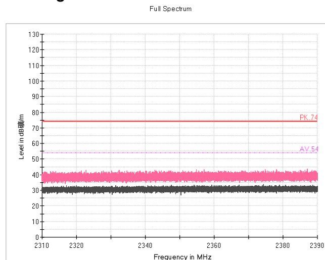
Radiated Emission Band Edge Channel No.:1 Test Mode: 802.11b Polarization: V
