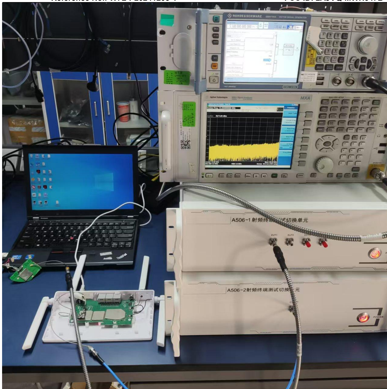
RF Conducted Test setup (DFS)
