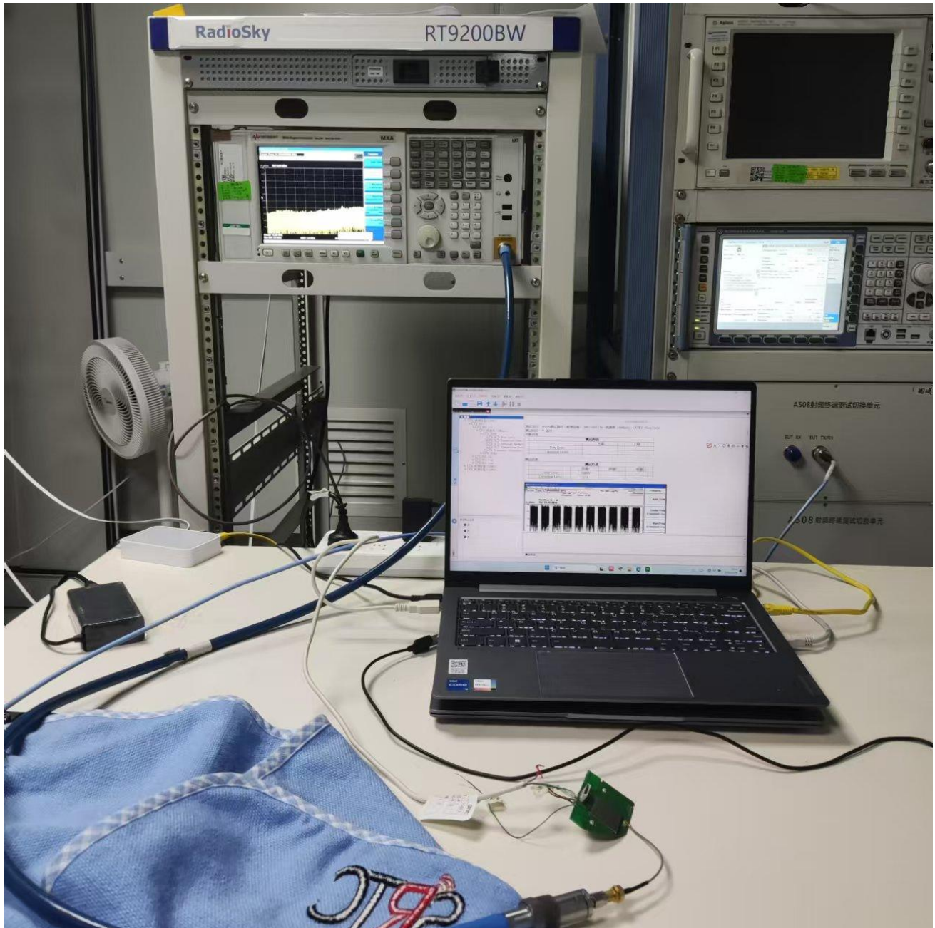
RF Conducted Test setup (WIFI)
